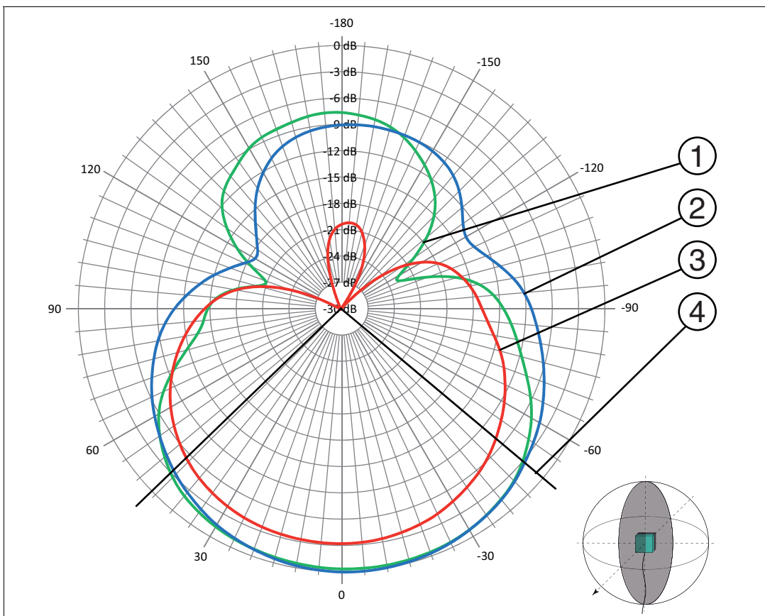
Figure 10.4 ① - Horizontal polarization ② - Vertical polarization ③ - Circular polarization with linear tag ④ - Full width at half maximum
