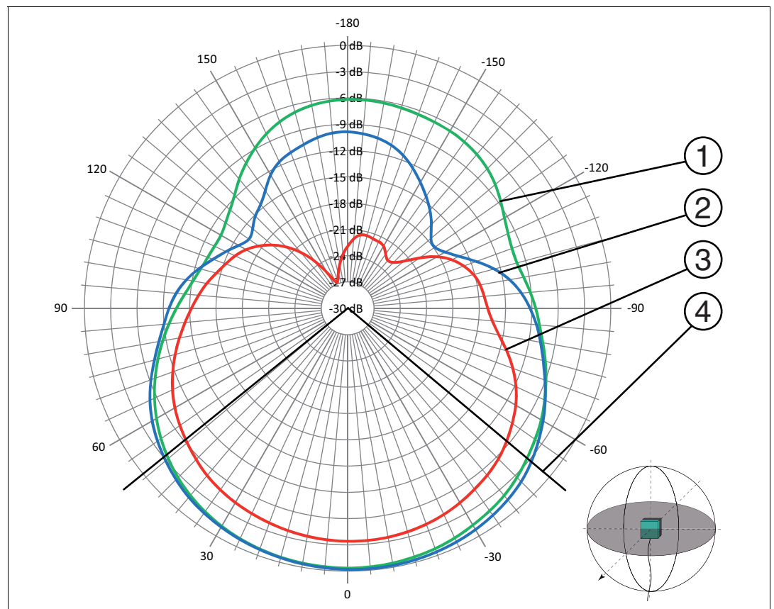
Figure 10.3 ① - Horizontal polarization ② - Vertical polarization ③ - Circular polarization with linear tag ④ - Full width at half maximum
