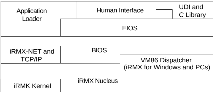
Figure 1-1. Layers of the iRMX OS
