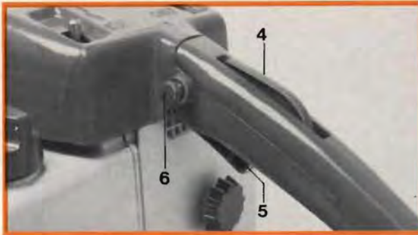
Starting-throttle position
