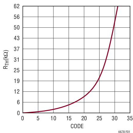
Figure 1. Programmable R_{COMP}
