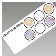
Color Slide II Mononucleosis test card w/positive and negative reactions.
