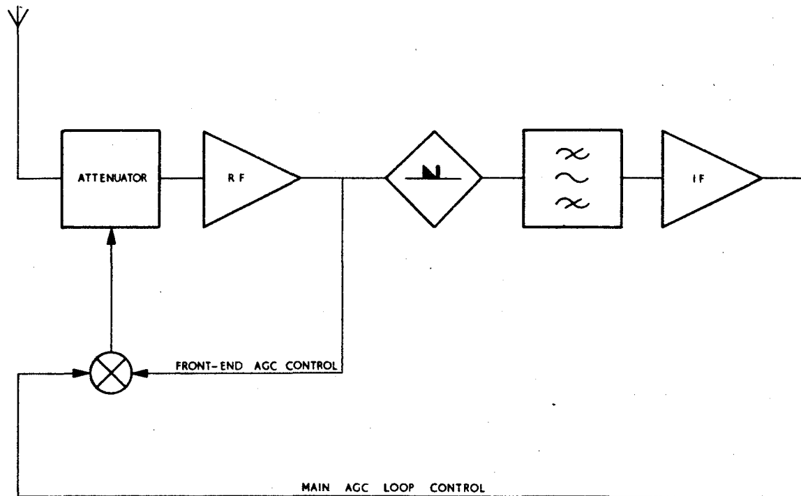
FIG. 6.4 AGC SYSTEM
