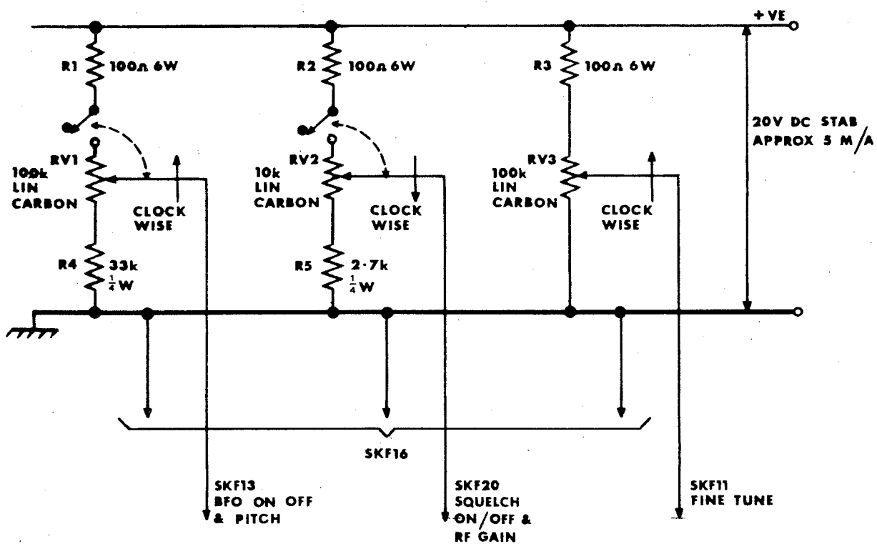
FIG.2 REMOTE CONTROLS
