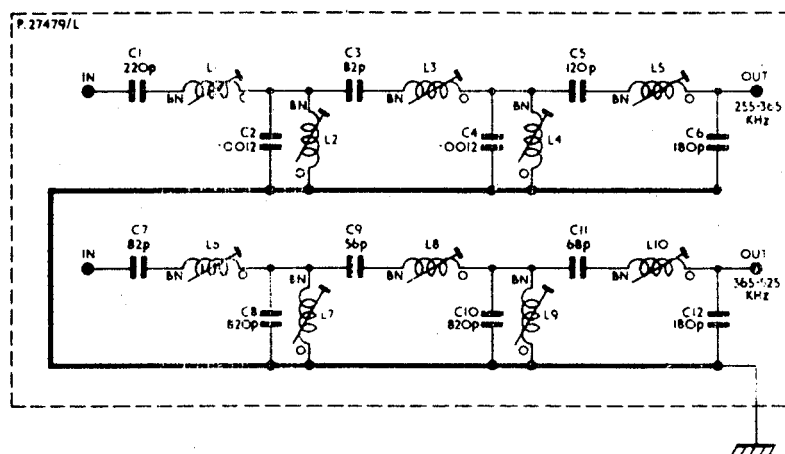
FIG. 6.1 MF FILTER
