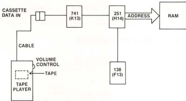
Fig. 4-61. Circuitry affected.
