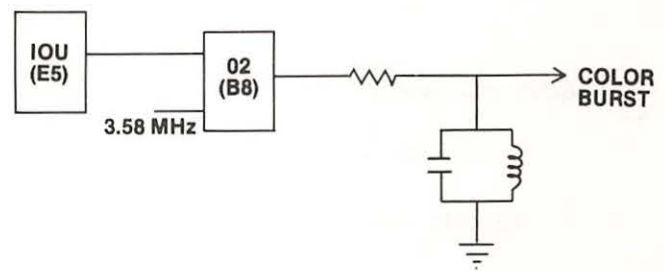
Fig. 6-15. Color burst circuitry.
