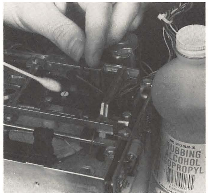
Fig. 8-11. This way to clean your read head is dangerous unless you wrap the cotton swab with a lint-free material.
