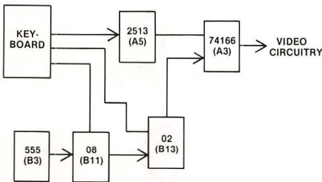
Fig. 4-37. Circuitry affected.
