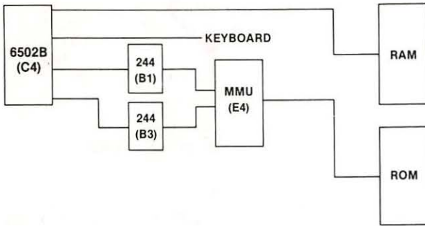
Fig. 7-21. Circuitry affected.
