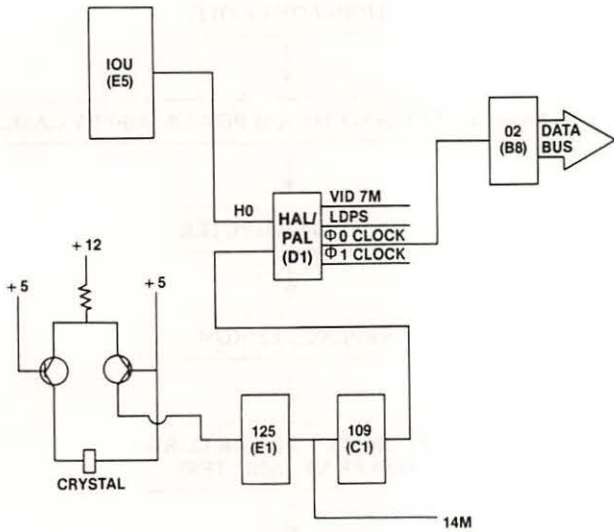
Fig. 7-3 Clock circuitry.
