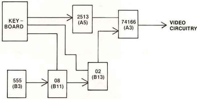
Fig. 4-53. Circuitry affected.
