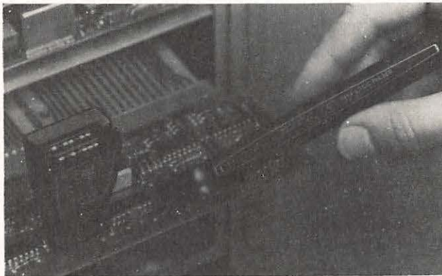
Fig. 9-5. A logic pulser can be used to inject a signal into a circuit.
