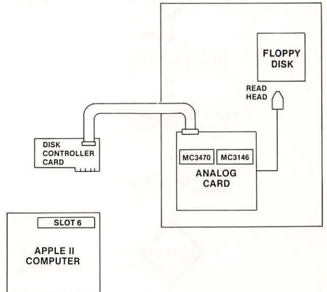
Fig. 7-20. Circuitry affected.
