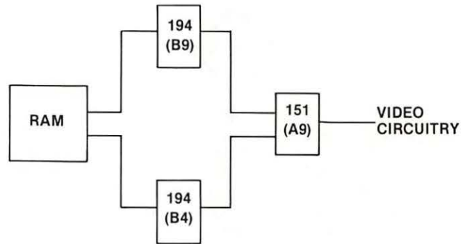
Fig. 4-23. Circuitry affected.
