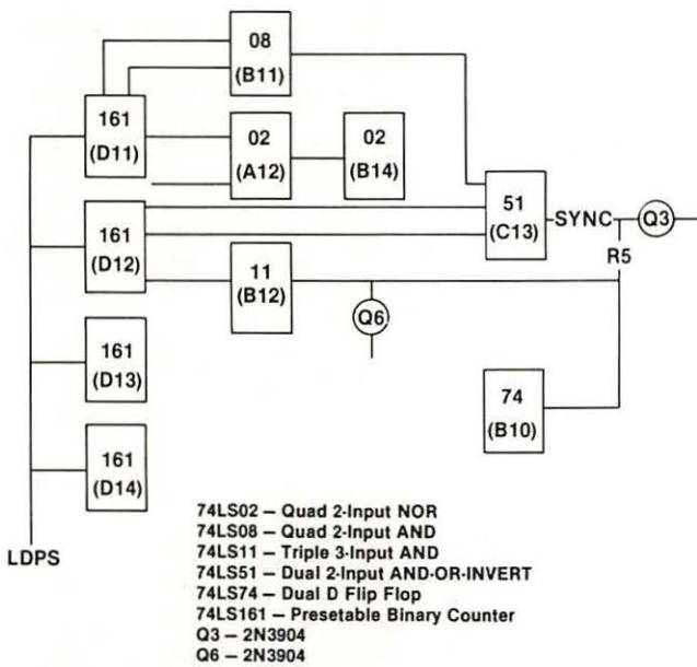
Fig. 3-14. Video display circuitry.
