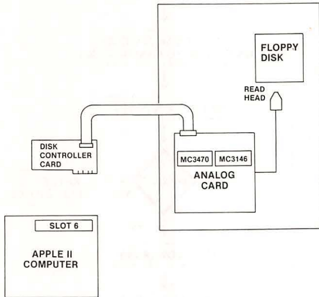
Fig. 4-16. Circuitry affected.
