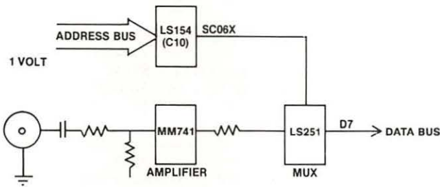
Fig. 7-59. Circuitry affected.
