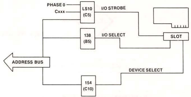
Fig. 7-67. Circuitry affected.
