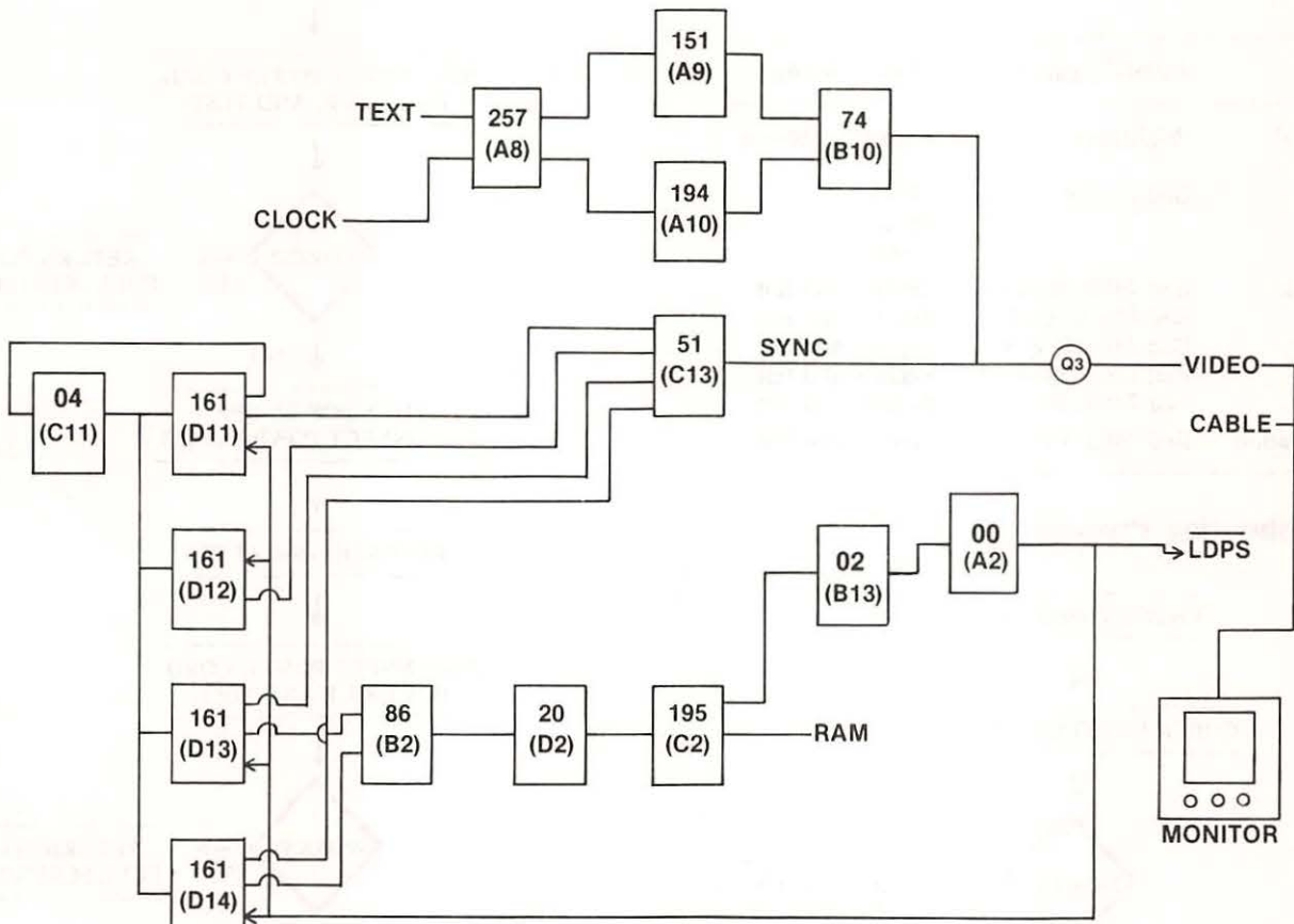
Fig. 4-25. Circuitry affected.
