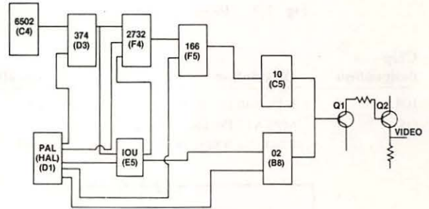
Fig. 7-5. Video circuitry.
