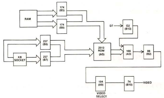
Fig. 4-49. Circuitry affected.
