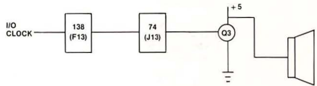
Fig. 4-7. Beep circuitry.
