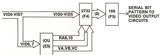
Fig. 7-37. Circuitry affected
