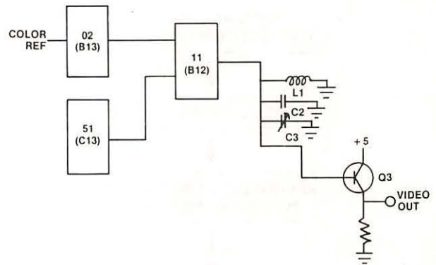
Fig. 4-29. Circuitry affected.
