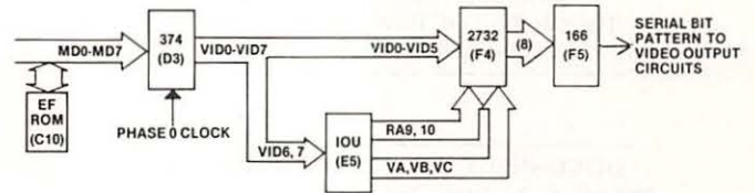
Fig. 7-33. Circuitry affected.
