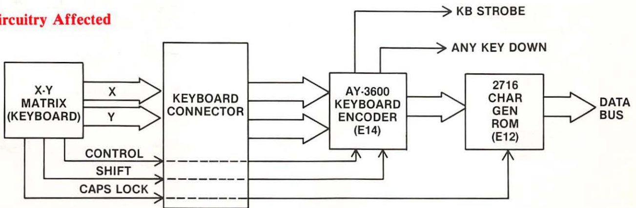
Fig. 7-45. Circuitry affected.
