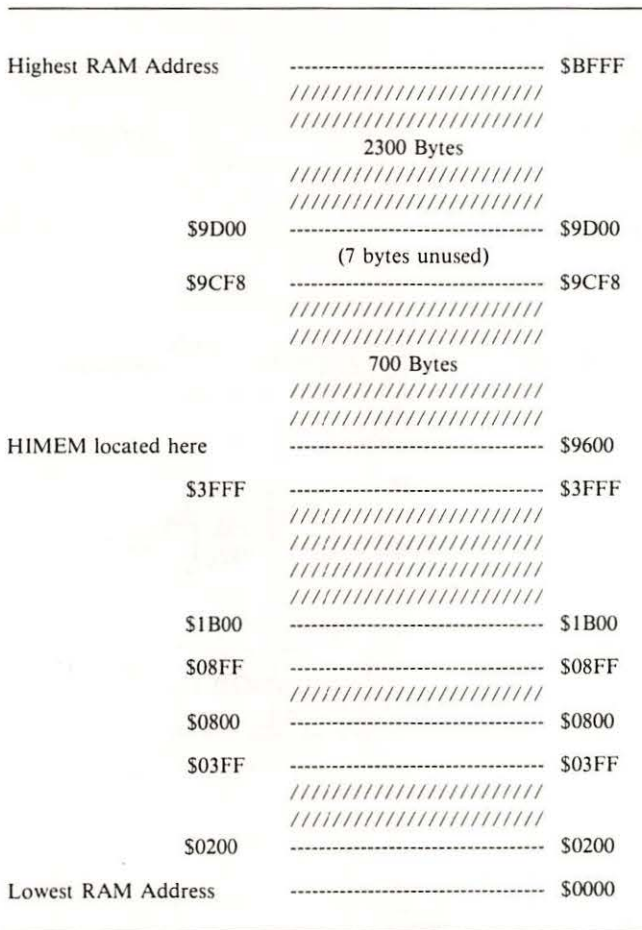
Fig. 6-7. RAM used during the DOS boot process.
