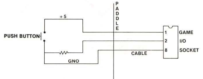
Fig. 7-65. Circuitry affected.
