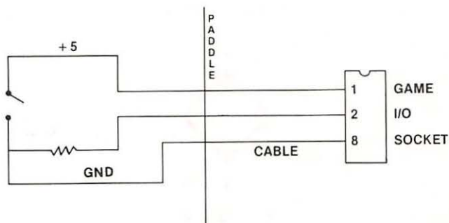
Fig. 4-67. Circuitry affected.
