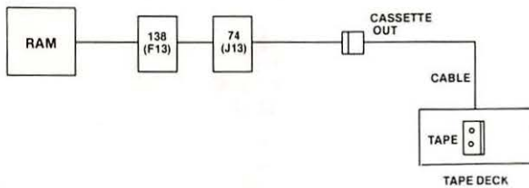
Fig. 4-63. Circuitry affected.
