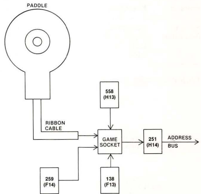
Fig. 4-65. Circuitry affected.
