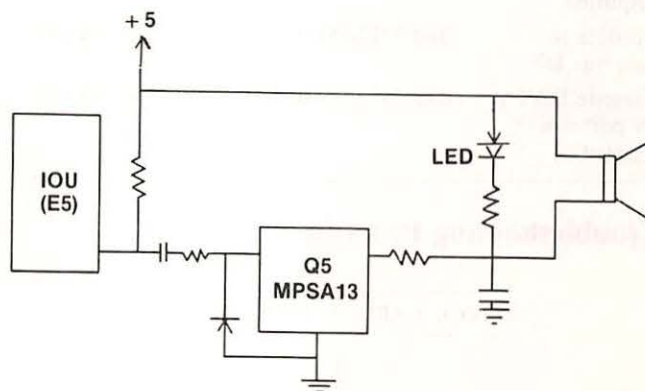
Fig. 7-57. Circuitry affected.
