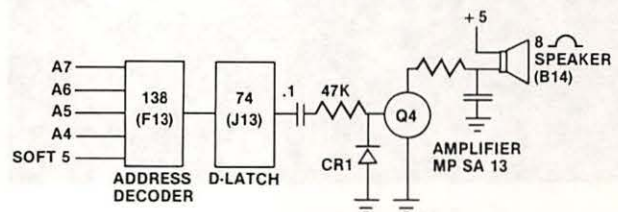
Fig. 3-23. Speaker circuitry.
