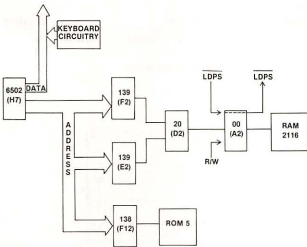
Fig. 4-21. Circuitry affected.
