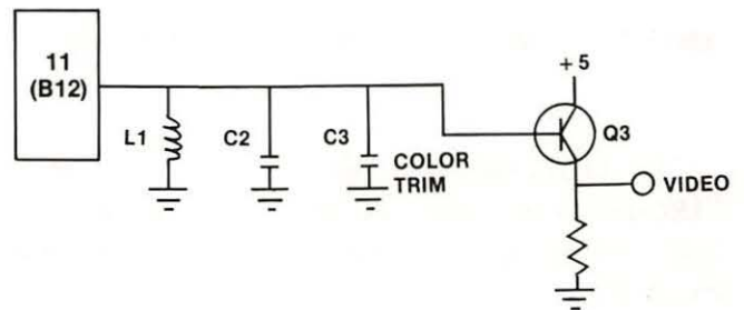
Fig. 3-16. The color-burst circuitry.
