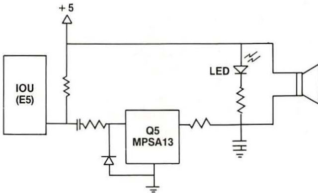
Fig. 7-7. Beep circuitry.
