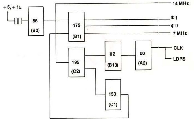
Fig. 4-3. Clock circuitry.
