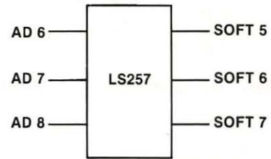
Fig. 3-15. Addresses are used to produce software switches.
