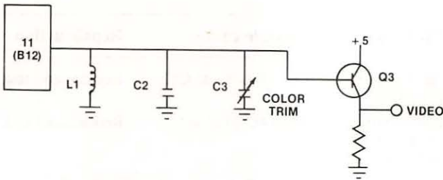
Fig. 4-41. Circuitry affected.
