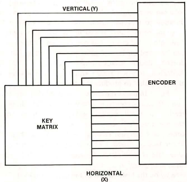
Fig. 3-21. Keyboard circuitry.
