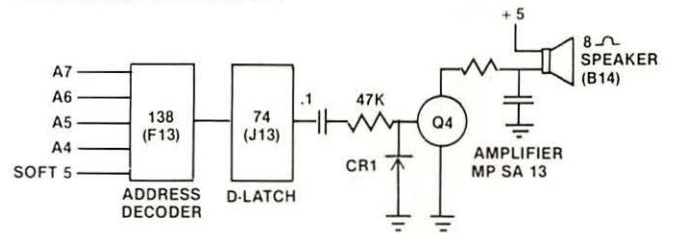
Fig. 4-57. Circuitry affected.
