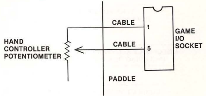
Fig. 4-68. Circuitry affected.
