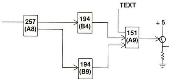
Fig. 4-43. Circuitry affected.
