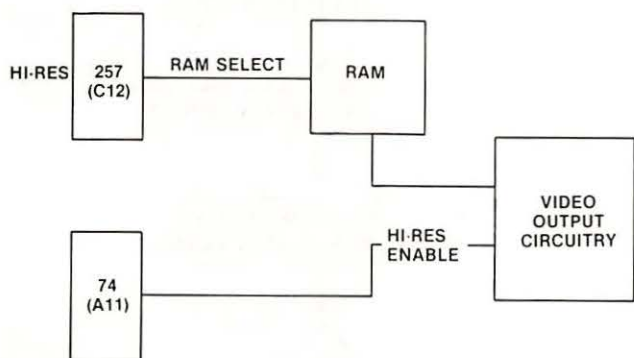
Fig. 4-45. Circuitry affected.
