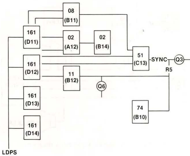
Fig 4-5. Video circuitry.
