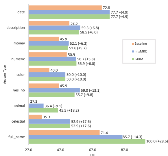
Figure 5: EM results comparison on M-BERT (MTQA French test set) for the different answer types.
