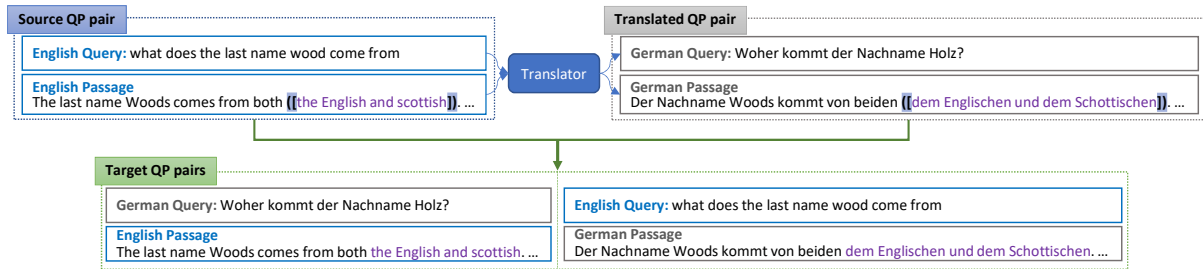
Figure 2: MixMRC data generation process. Given source (English) QP pair, we translate QP pair from English into non-English. Then the target mix-language pair can be divided into two forms: translated question-source passage and source question and translated passage pair.
