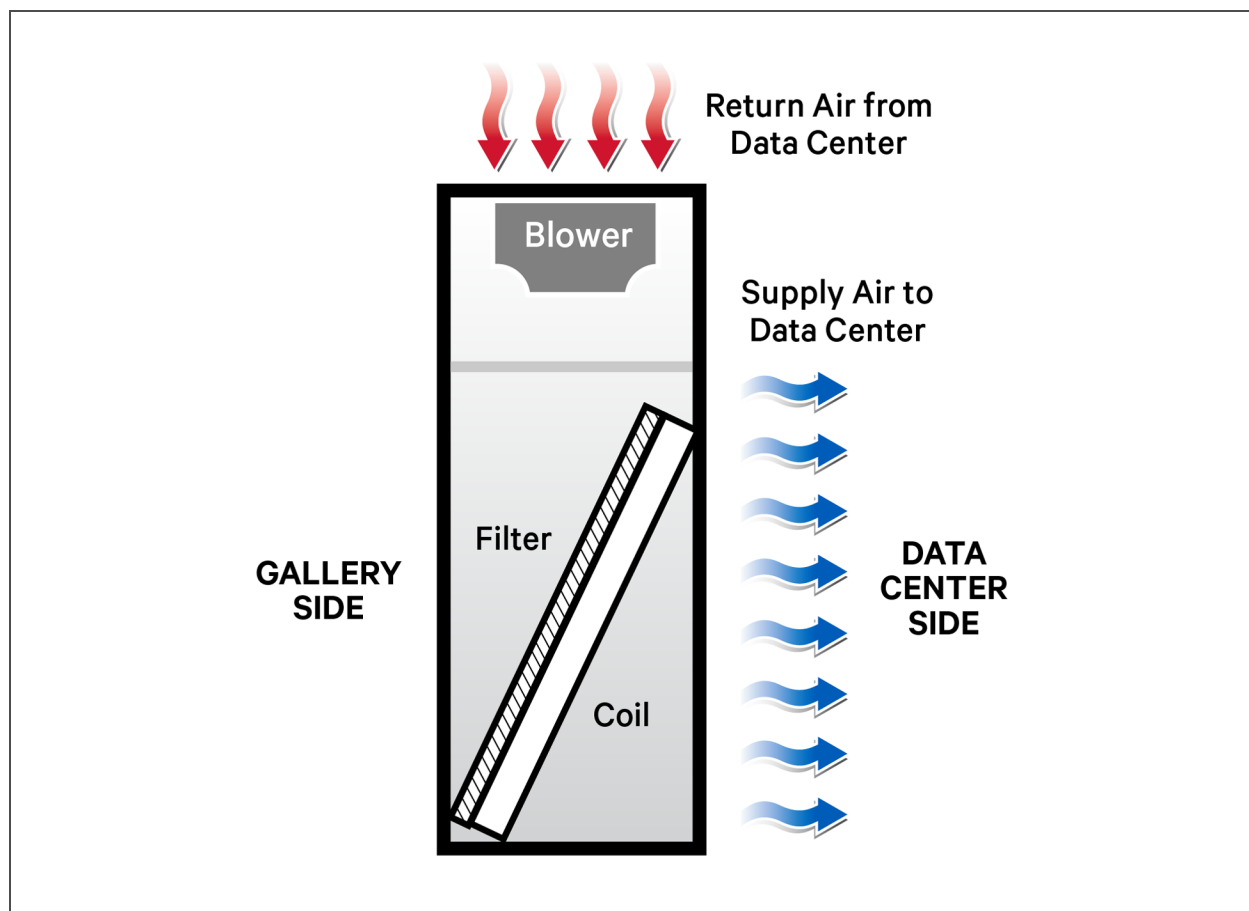
Figure 1.1 Downflow, horizontal-discharge blower configurations with EC fans
