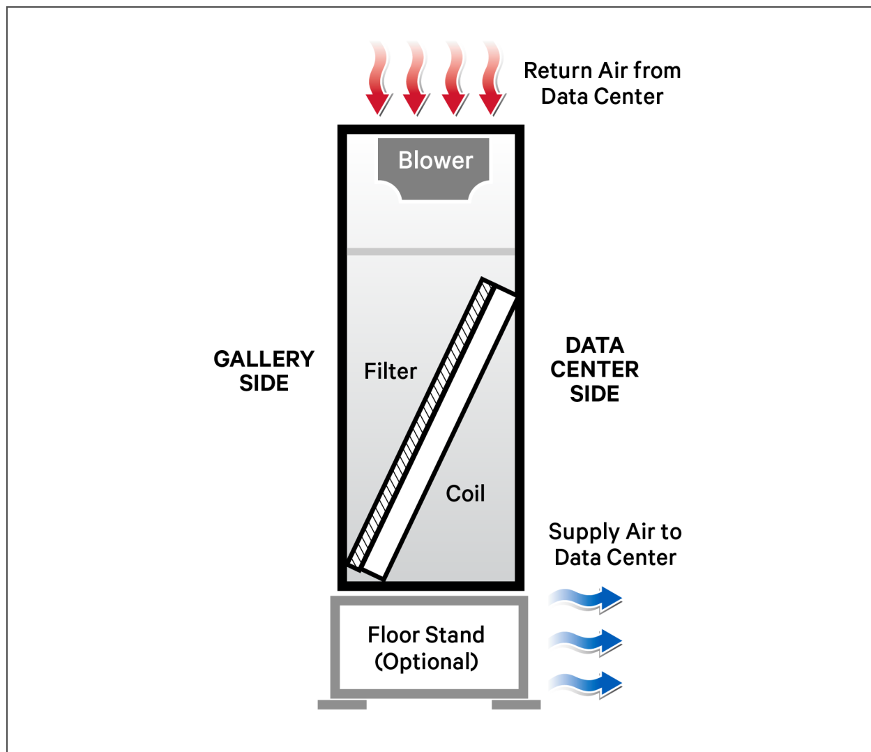
Figure 1.3 Downflow, bottom-discharge blower configurations with EC fans
