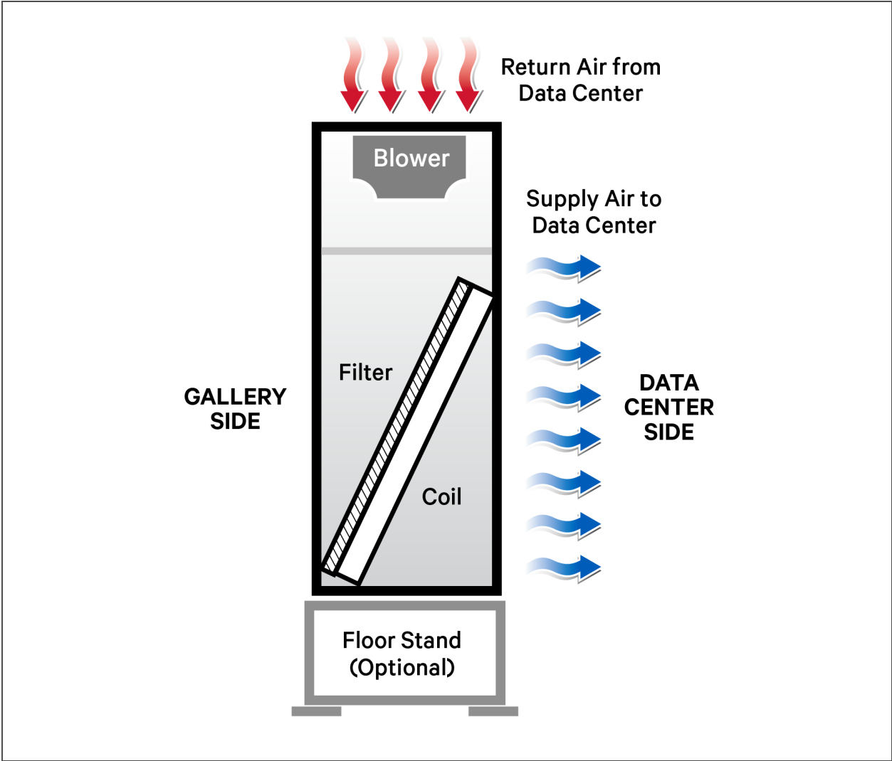
Figure 1.2 Downflow, horizontal-discharge blower configurations with EC fans on a floor stand
