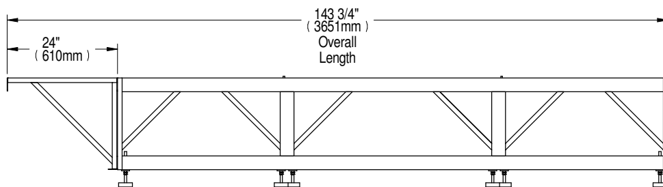
60" ( 1524mm ) Overall Depth A
