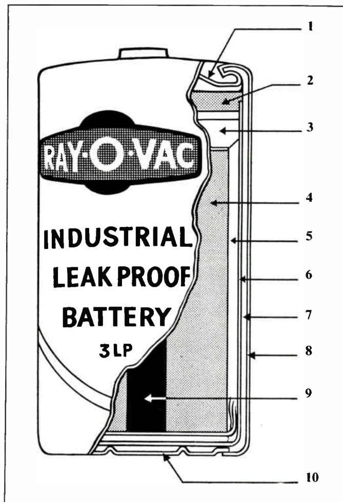
1. Steel top cap. 2. Plastic seal. 3. Air space. 4. Manganese dioxide. 5. Electrolyte. 6. Zinc. 7. Bitumen tube insulator. 8. Steel jacket. 9. Carbon rod. 10. Steel bottom plate.
