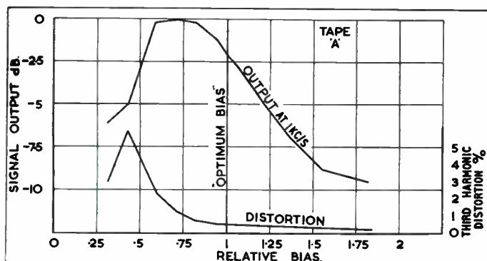
Fig. 1. Displays "optimum bias". The lower curve shows the third harmonic distortion factor, and the upper curve shows the output, as bias is altered.
