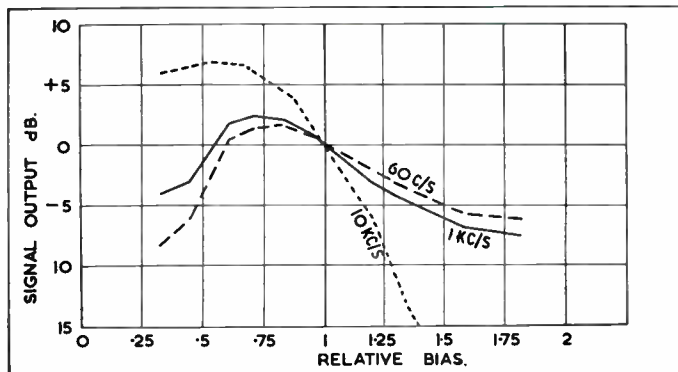
Fig. 3. Shows the erasure effect of the H.F. bias. Three "spot" frequencies, recorded at the same input level, indicate a more marked effect on higher frequencies than on low.
