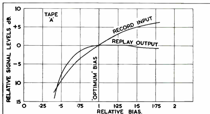
Fig. 2. Shows how change of bias also changes tape sensitivity.
