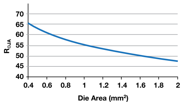
Figure 6. Package R_{\theta JA} vs. die area. As the die area shrinks, the associated R_{\theta JA} gets exponentially worse.
