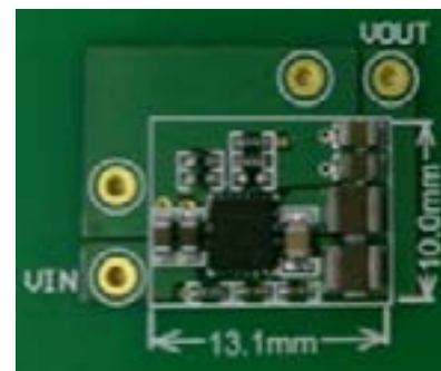
Figure 3. A 10-A point-of-load converter measuring 13.1 mm by 10 mm in area, resulting in 76 mA/mm 2 of current density.
