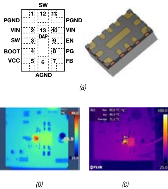
Figure 10. Enhanced HotRod QFN with a large DAP to improve thermal performance (a); thermal performance of a conventional HotRod package (b); thermal performance of the enhanced HotRod QFN with DAP product (c).
