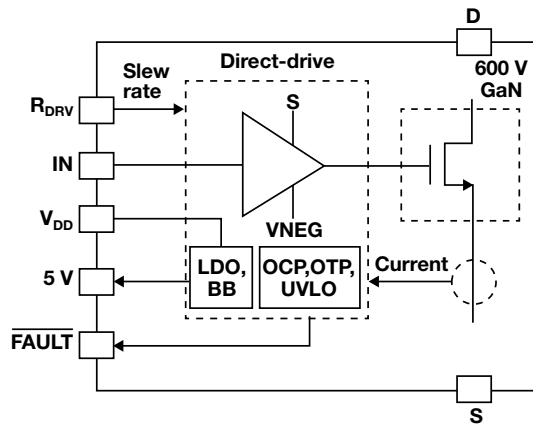
Figure 16. Driver, protection and monitoring functions integrated with a GaN switch on the LMG3410.
