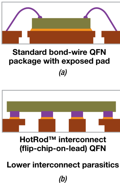
Figure 9. Standard QFN with bond-wires to electrically connect to the die (a); HotRod package with copper pillars and flip-chip interconnect between the leadframe and die (b).
