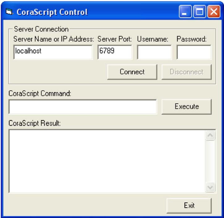
FIGURE 5-1. CsiCoraScript Example
