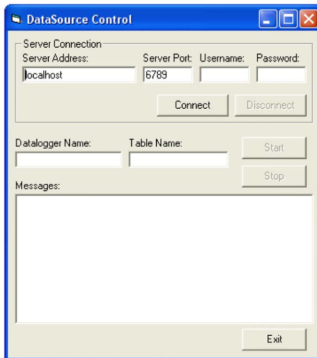
FIGURE 11-1. CsiDataSource Example
