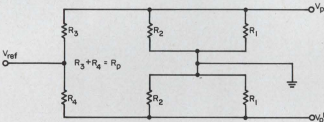
3. Equivalent circuit of the configuration in Fig. 3 simplifies analysis and yields design equations.
