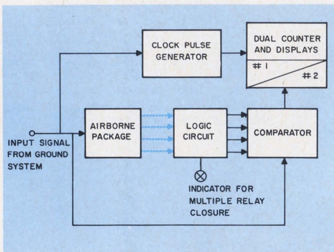
1. A telemetry link provides control/monitor path between the airborne package and the test system. A dual counter is used to display the test results. One clock signal triggers both airborne and ground systems.
