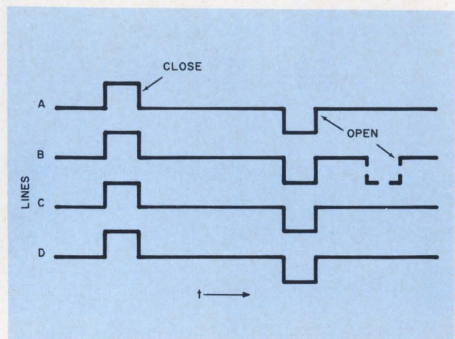
2. A binary-coded pulse input to the logic circuit. The solid lines indicate pulses associated with relay #11. The dotted pulse shows the only signal change required to identify relay #2.
