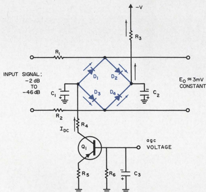
3. Controlled, balanced, L-pad is formed by the diode-bridge attenuator circuit. Input impedance of bridge is much higher than that of transformer, thus presenting constant impedance to line. L-pads are established by D_1 , D_2 and R_1 , and D_3 , D_4 and R_2 , respectively, acting with the transformer secondary. Transistor Q_1 is a control amplifier that establishes the conduction levels of the diodes.
