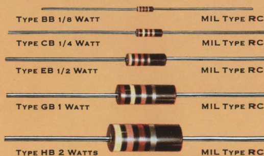
These are the same hot molded resistors as used in the hermetically sealed construction described above. Shown actual size.
