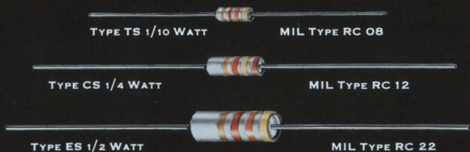
HERMETICALLY SEALED HOT MOLDED RESISTORS available in all standard EIA and MIL-R-11 resistance values and \pm 2\% or \pm 5\% tolerances. Other than standard values can be furnished. Shown actual size.
