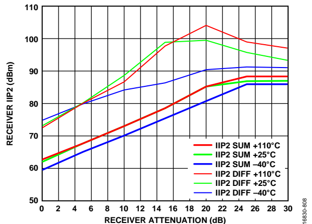
Figure 106. Receiver IIP2 vs. Receiver Attenuation, LO = 4600 MHz, Tones Placed at 4645 MHz and 4646 MHz, -21 dBm Plus Attenuation
