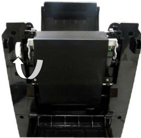
Loading path for ribbon
