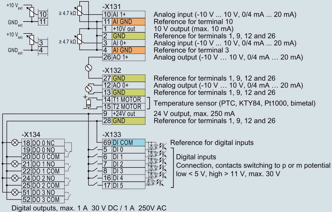
Connection example for SINAMICS G120XA
