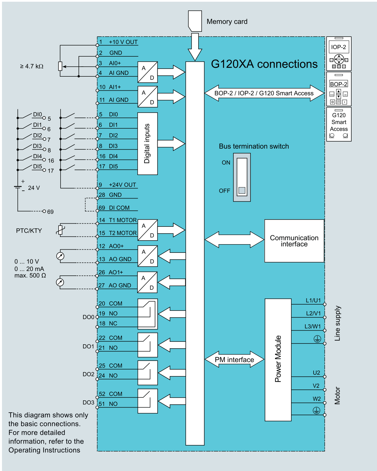
Block diagram SINAMICS G120XA
