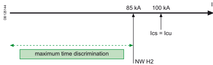
Limited time discrimination.
