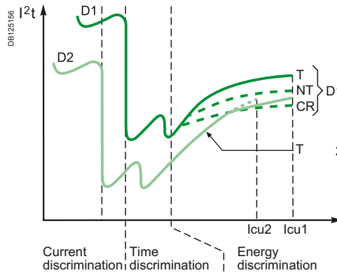
Discrimination enhanced by cascading: curves.
