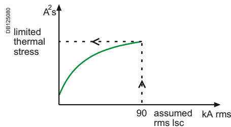
Thermal stress limitation curve.
