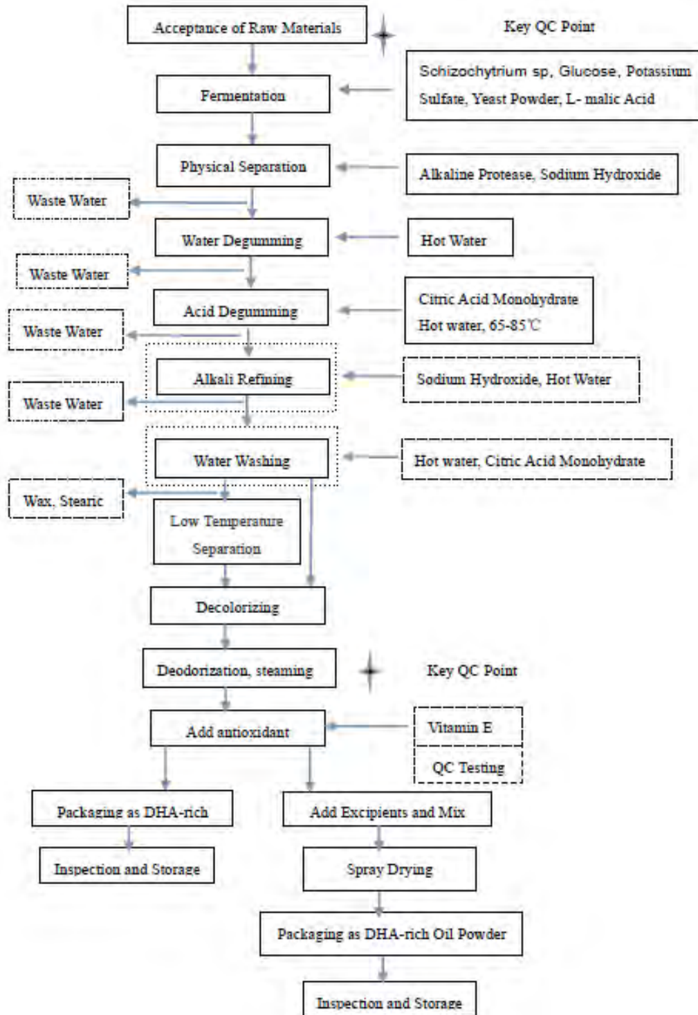
Figure 2. Manufacturing Flow Diagram of DHA-rich Oil Ingredients
