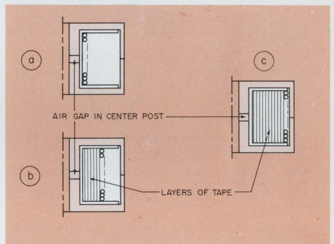
8. Three different winding configurations for a 1408 pot core wound with 15 turns of 12-44 Litz wire.
