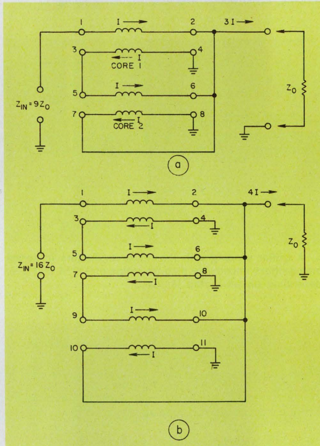
2. Two cores are required in a transmission-line transformer to achieve a 9:1 impedance ratio (a). Three cores are required for a 16:1 ratio (b).
