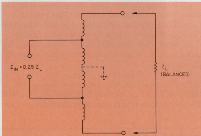
7. A quadrifilar winding offers a 0.25:1 impedance ratio, and the center-tap may be grounded.
