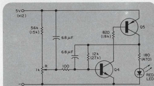
2. Ripple and noise voltages in power supplies can be detected over the range of 10 to 600 mV, peak-to-peak. Sensitivity is adjusted with potentiometer R.
