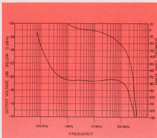
16. Transformer bandwidth is flat from 1 to 100 MHz, with an impedance transformation ratio of 9:1.
