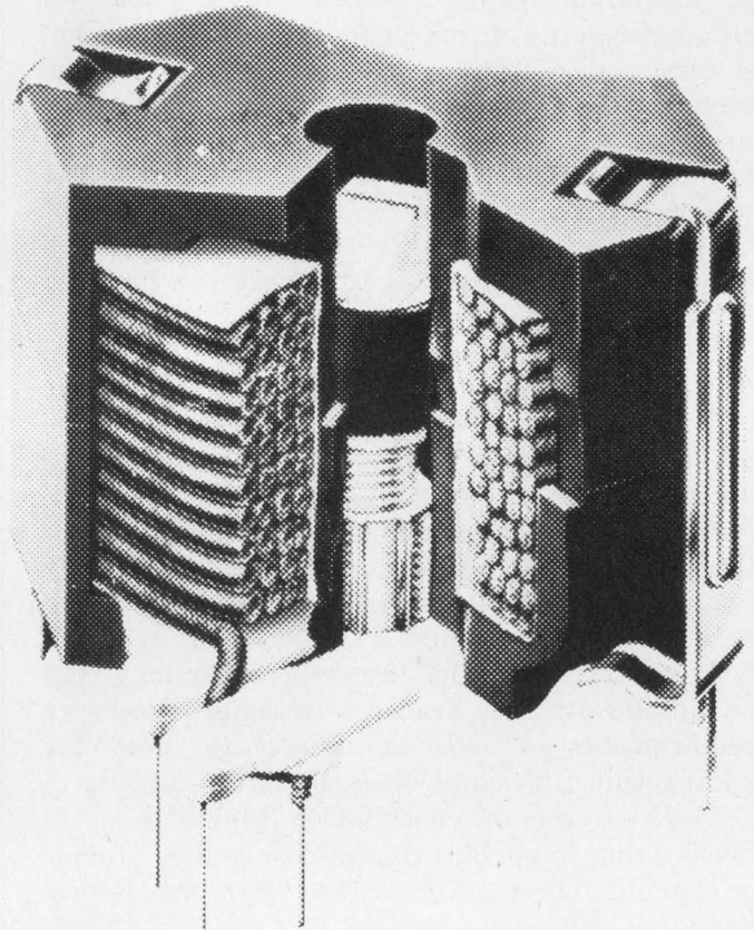
1. A ferrite pot core is completely self-shielding. Thus it eliminates worries about interference with nearby circuit components.
