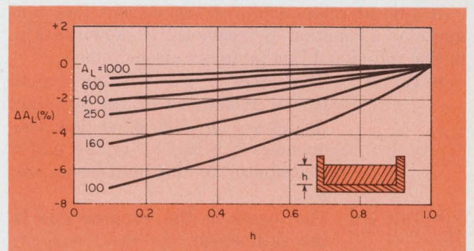
4. If less than the total bobbin height is used, the actual inductance will be lower than the calculated value. The larger the air gap, the greater the deviation.
