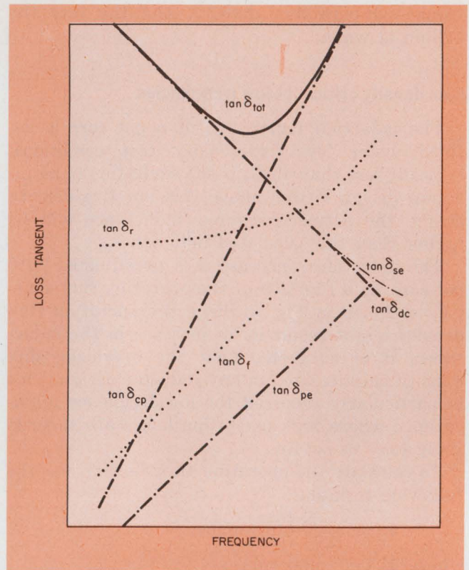
6. Typical variation of contributory loss tangents as a function of frequency. The total loss tangent is the sum of all the contributory loss tangents.
