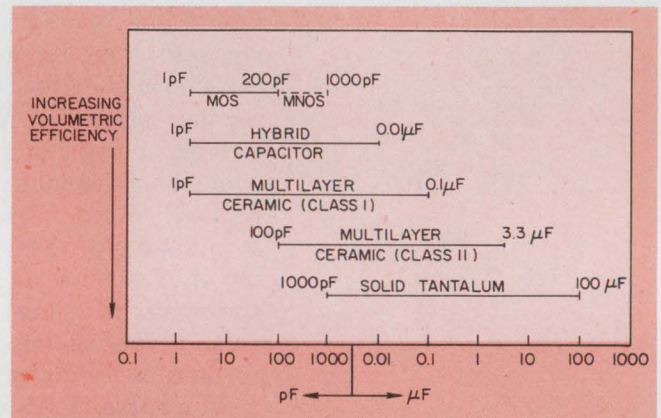
1. Capacitance ranges and volumetric efficiencies available for hybrid subassemblies.
