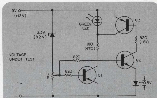
1. A voltage-limit sensing circuit lights a LED when the voltage is within 0.5 V above the limit set by potentiometer R. Values shown in brackets are for 12-V operation.
