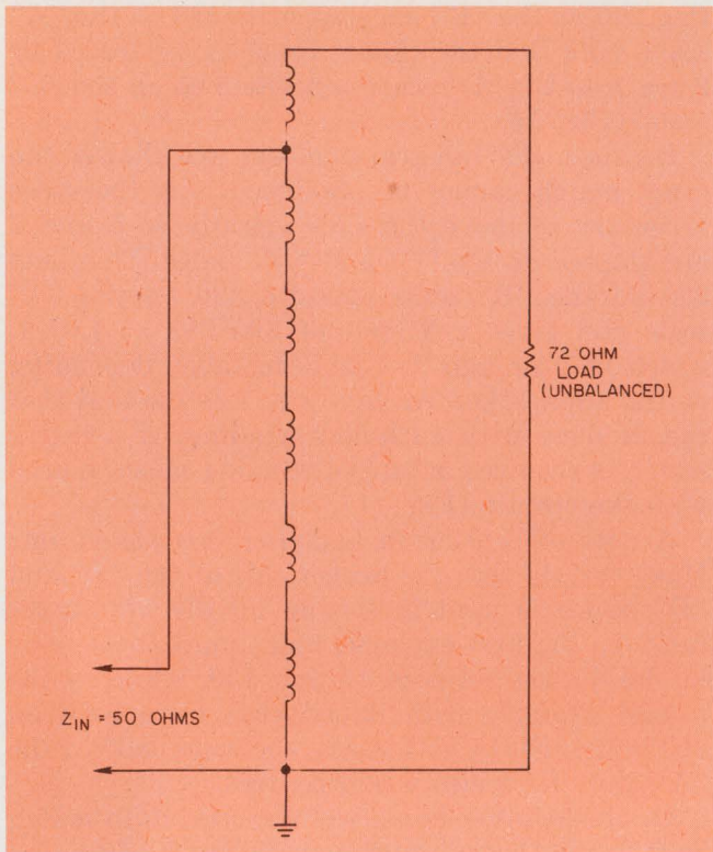
9. A hexafilar winding is used in this example to match a 72-Ω load to a 50-Ω cable.
