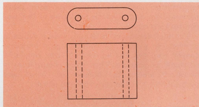
14. A balun core is the form that results when two toroidal coils are placed side by side.
