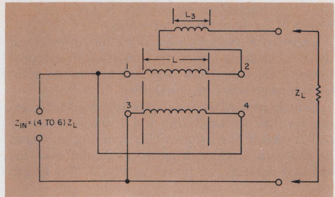
3. To extend a 4:1 impedance ratio to 6:1, a third winding, L_3 , is wound over the original winding, L .
