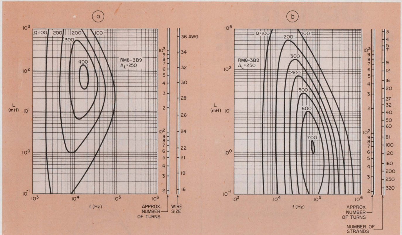
7. Iso-Q curves illustrate the effect of wire size on attainable Q. Typical Q curves obtainable with solid mag-
