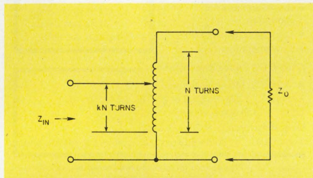
1. In a basic autotransformer used for impedance step-down, Z_{in} = k^2 Z_{out} where k is the location of the tap.
