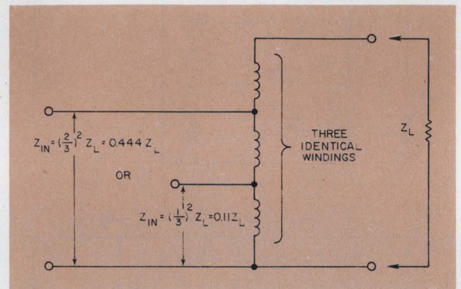
4. A trifilar winding with the three conductors in series aiding offers impedance step-up ratios of 1:9/4 and 1:9 , depending on which tap is used.
