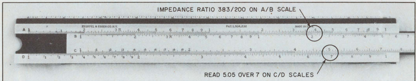
10. Slide-rule algorithm for finding turns ratio to match 200 to 383 Ω, both balanced to ground.
