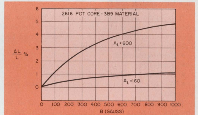
3. An increase in operating flux density will result in an increase in inductance value.
