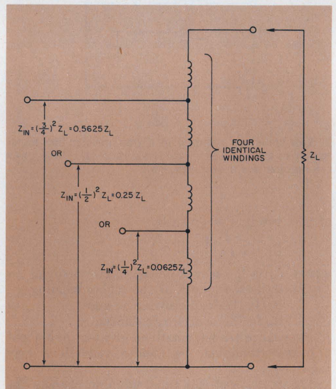
5. A quadrifilar winding can extend impedance ratios to 1:(4/3)^2 , 1:4 and 1:16 , depending on the tap.
