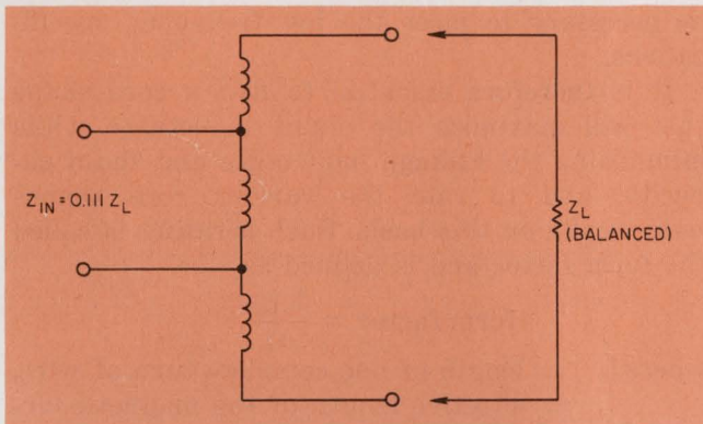
6. A trifilar transformer provides a 0.111-to-1 impedance ratio in a balanced-to-balanced transformation.
