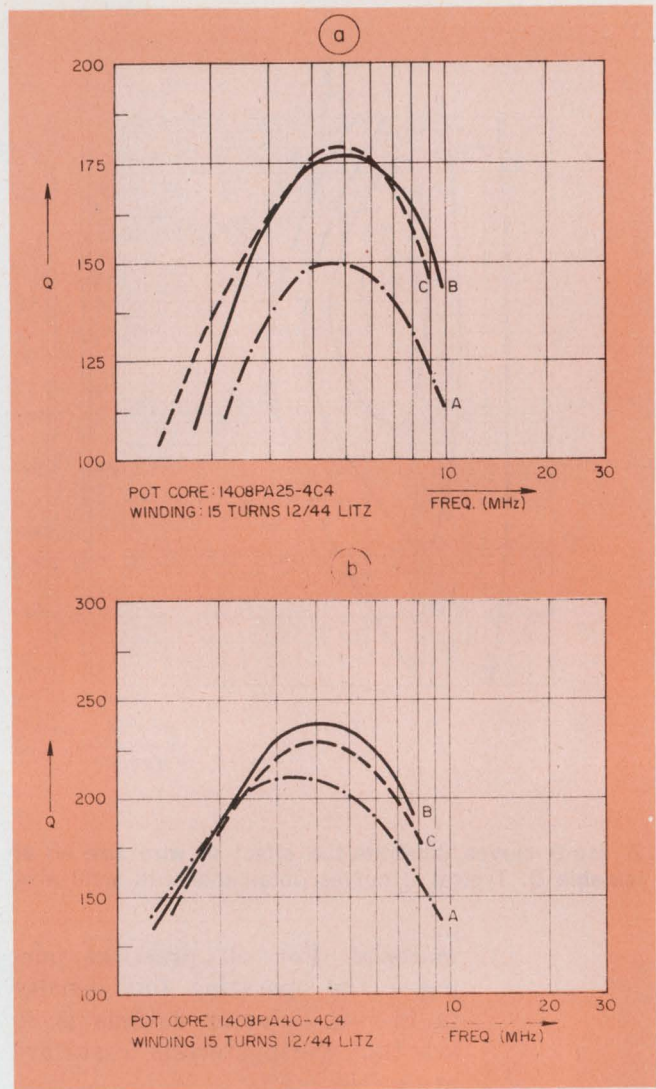
9. Q curves measured on two 1408 pot core sets in 4C4 nickel zinc material with A_L of 25 (a) and A_L of 40 (b).
