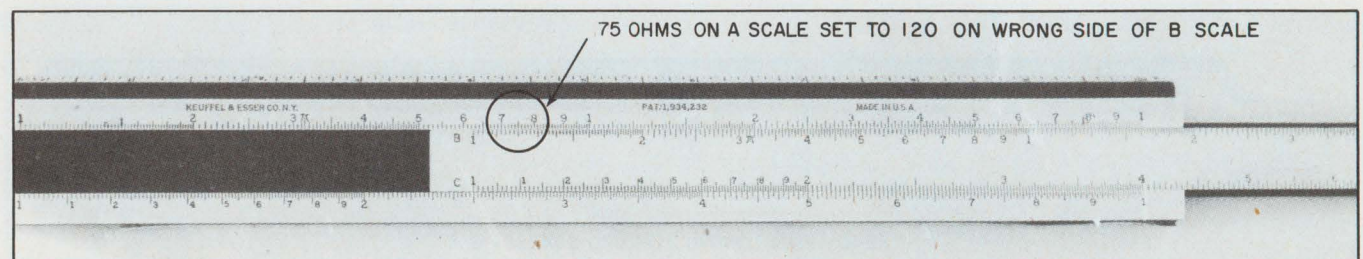
12. An incorrect turns ratio will appear if the wrong half of the A or B is used.
