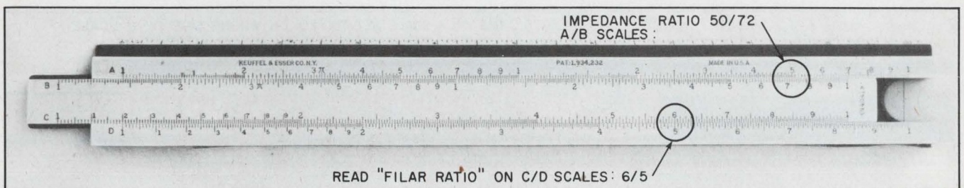
8. Slide-rule algorithm for determining turns ratio for matching 50 to 72 \Omega , unbalanced.
