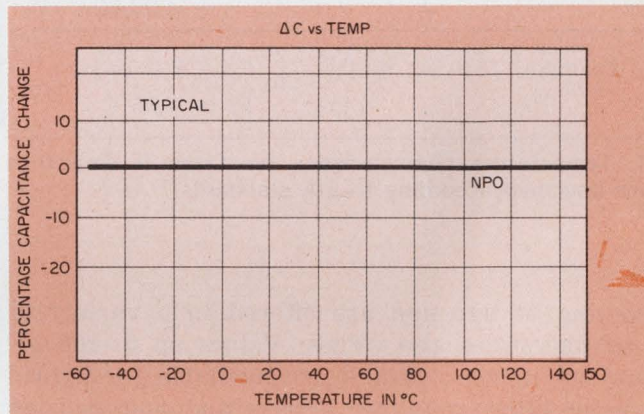
3. Class I NPO dielectric capacitors are available with a guaranteed \pm 30 ppm/ ^{\circ}\text{C} drift from -55 C to +125 C.
