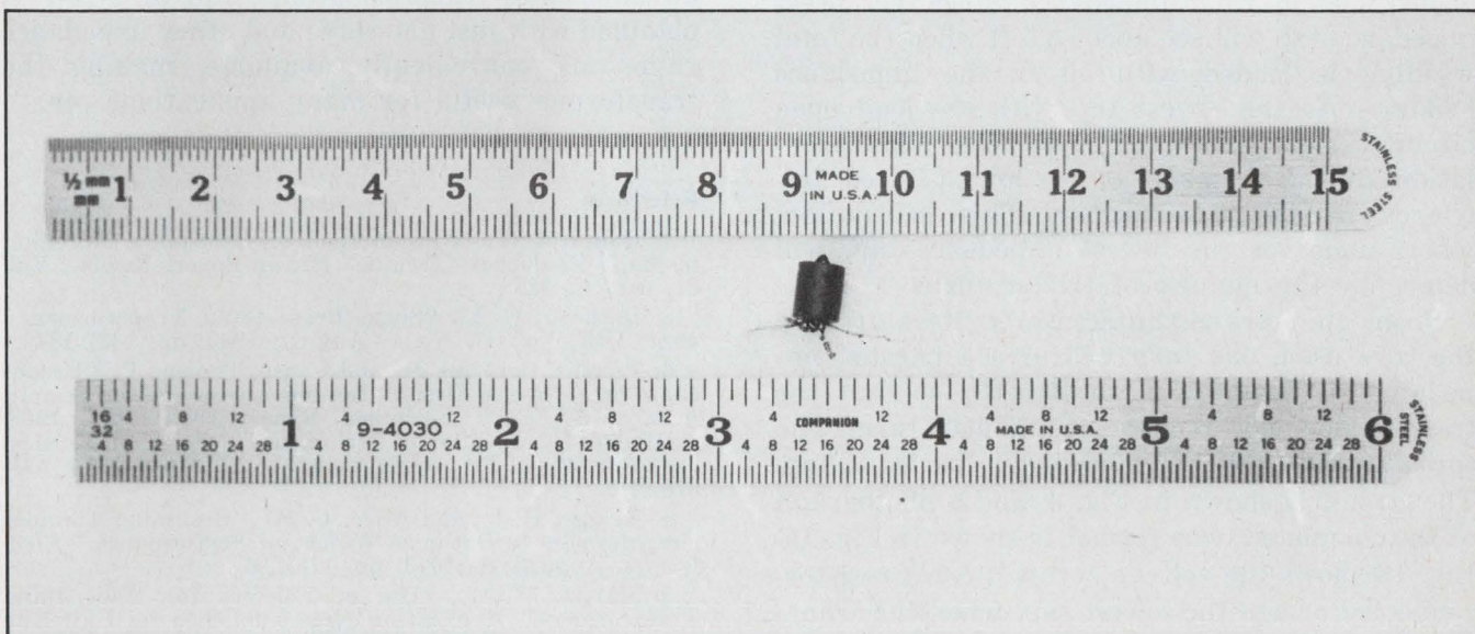
15. The compact 5.5-Ω to 50-Ω transformer uses a trifilar winding, with the strands connected series-aiding.
