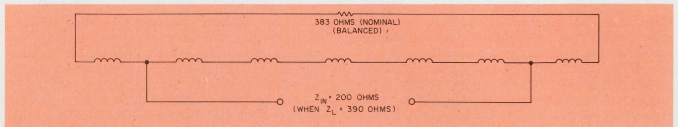
11. A seven-winding autotransformer is needed to match 383 to 200 Ω, both balanced to ground.
