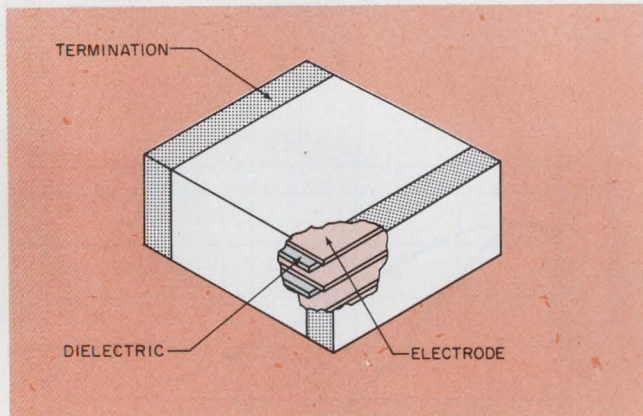
2. Multilayer ceramic capacitors are fabricated by stacking and co-firing thin sheets of metalized green dielectric.
