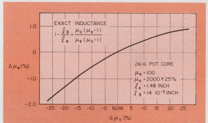
2. An air gap is used in a pot core to reduce the wide tolerance on initial permeability ( \mu_o ). Here a \pm 25\% initial-permeability tolerance is reduced to -1.8\% to +1\% tolerance in effective permeability ( \mu_e ).
