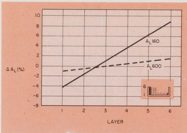
5. The position of layers of turns on a pot core introduces still another deviation between actual and calculated values. Layers 1 and 2 have less than average inductance, while layers 3 to 6 have more than average inductance per turn.
