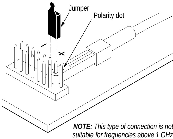
Figure 4: Using a square pin and jumper
