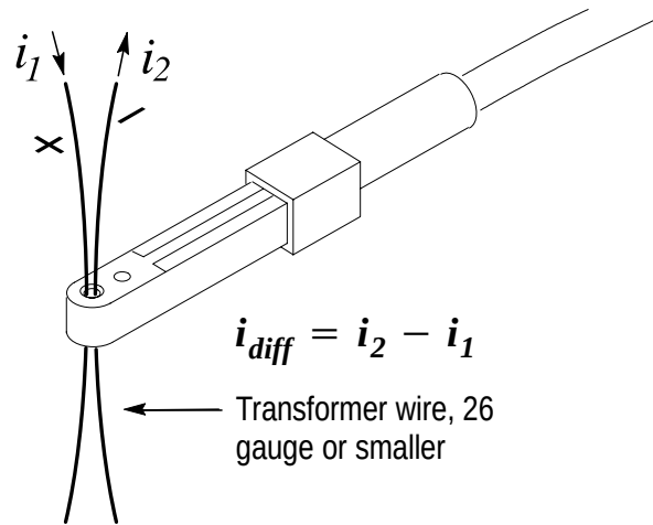
Figure 3: Using two wires to measure differential current
