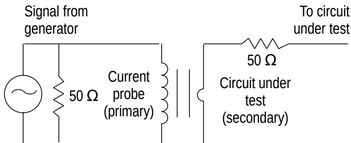
Figure 7: Signal injection
