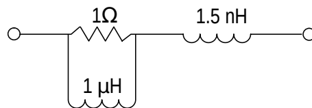
Figure 8: Circuit equivalent of added inductance and capacitance
