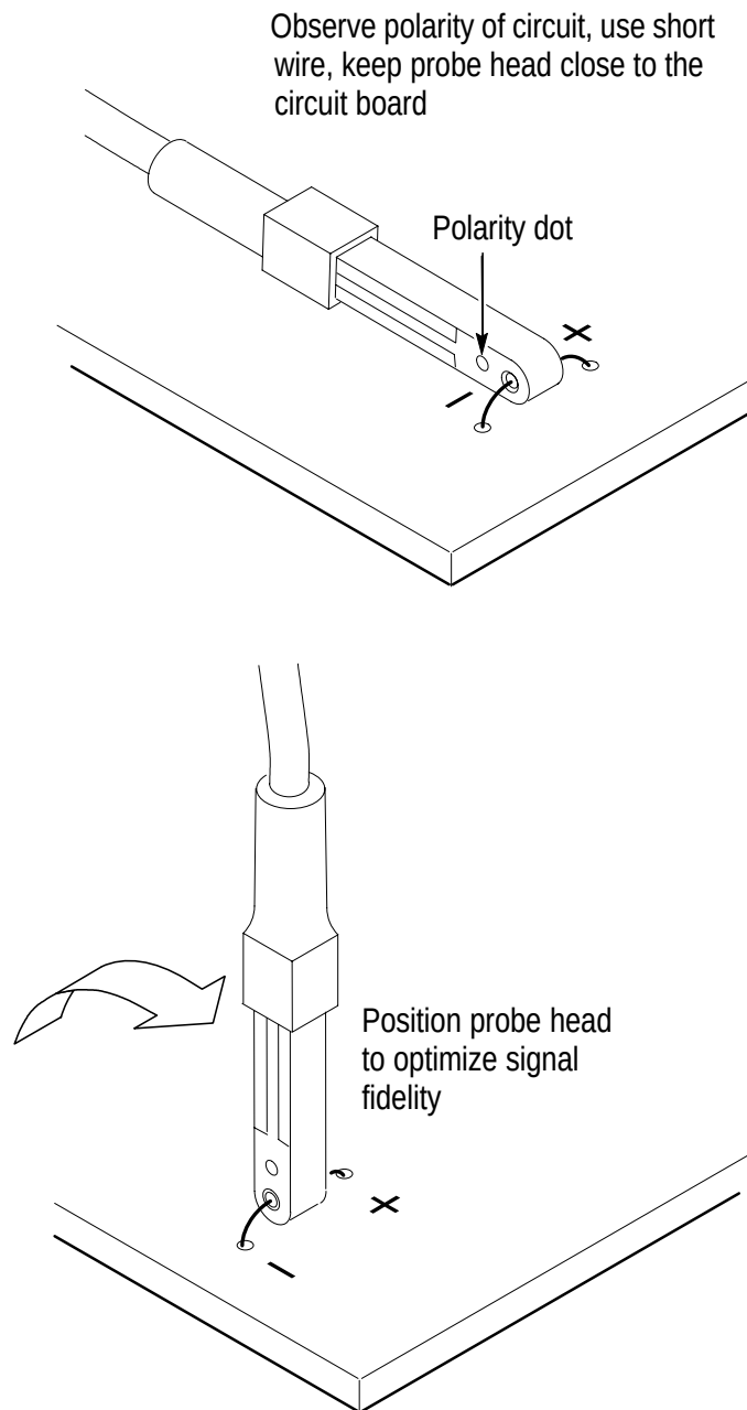
Figure 2: Using a single wire
