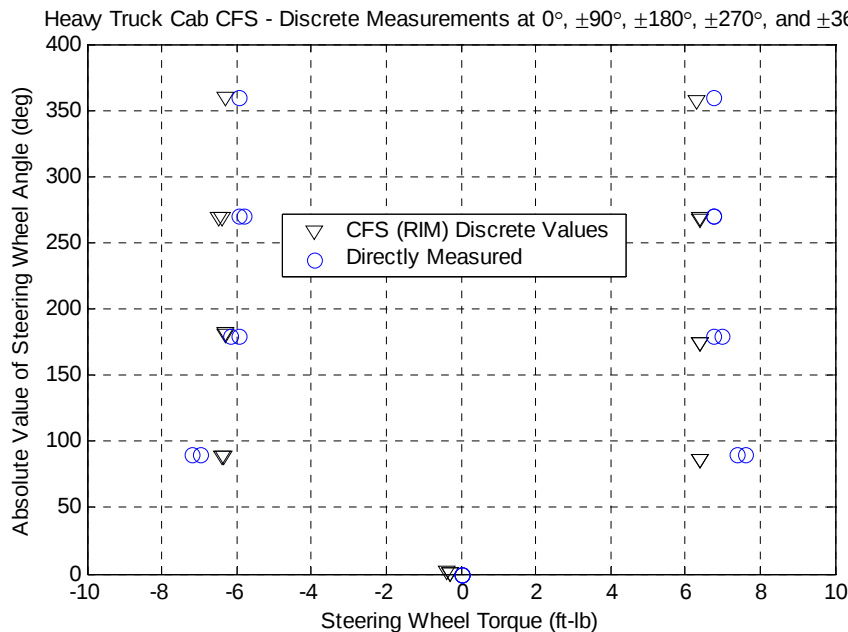
Figure F1 - Direct and CFS Measurements of Discrete Steering Properties
