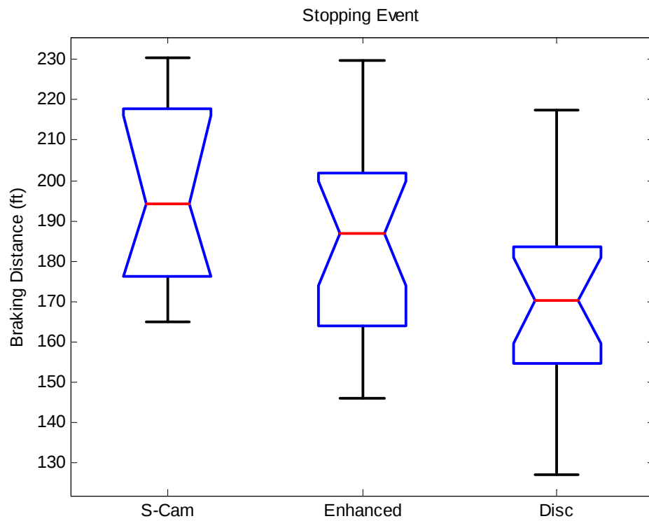
Figure A20 - Stopping event braking distance
