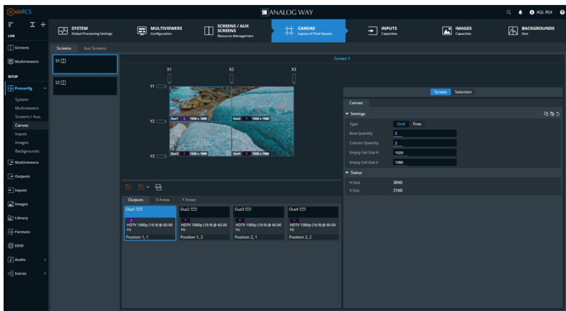
Fig. 10 - Preconfig - Canvas
