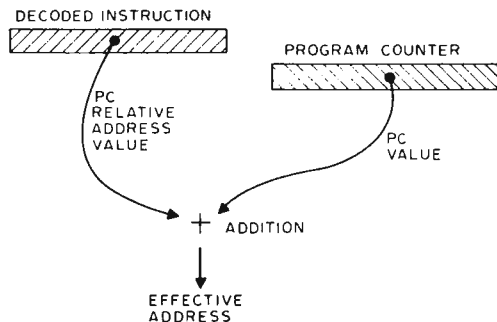
Figure 7: Program Counter Relative Addressing. Some computers provide a means to address memory in terms of an address displacement relative to the current program counter value. The instruction contains the displacement which the processor adds in the current program counter value for this type of effective address calculation.
