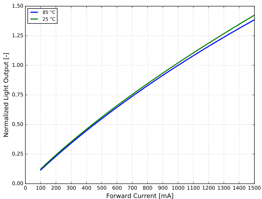
Figure 3b. Typical normalized light output vs. forward current for LUXEON FX2-L Plus Cool White at < 20 ms MP, 25°C and 85°C.
