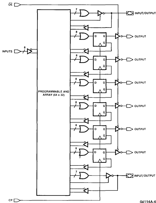
AmPAL16R6L BLOCK DIAGRAM
