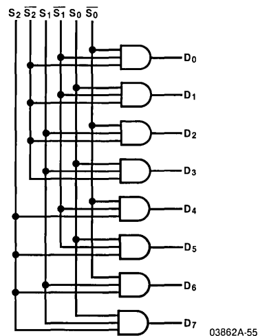
(c) Logic Diagram 3-to-8 Decoder
