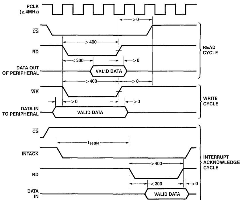
Figure 2. Am8500 Interface Timing (4MHz)
