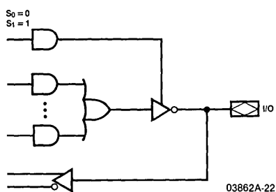
Combinatorial/Active LOW Configuration
