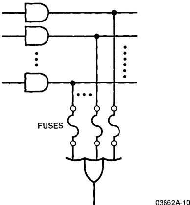
Figure 3b. Programmable OR Array Logic Equivalent
