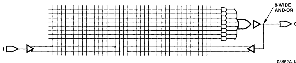
Figure 9b. Active HIGH Dedicated Output
