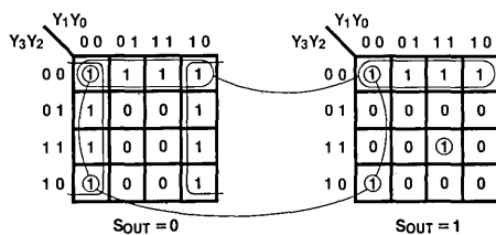
Figure 6. INV Flag Mode Definitions
