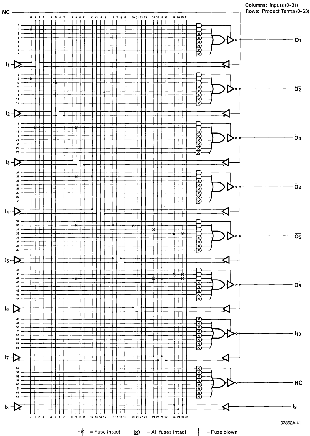
Figure 4. Logic Diagram for Function of Figure 1 Using the AmPAL16L8
