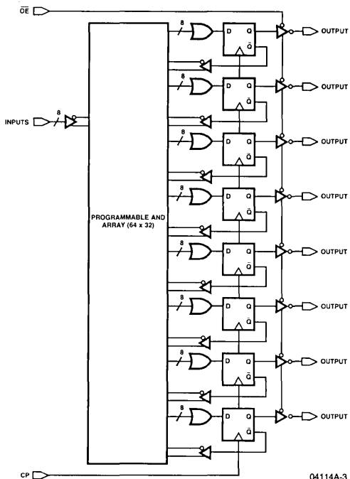
AmPAL16R8L BLOCK DIAGRAM
