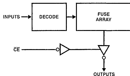
Figure 1. PROM
