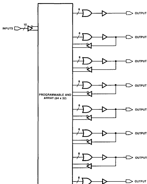
AmPAL16HD8L BLOCK DIAGRAM
