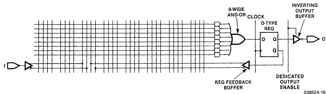
Figure 8. Registered Output
