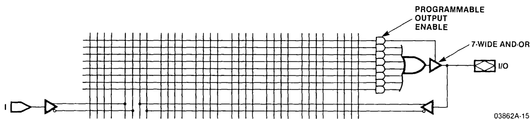
Figure 7b. Active HIGH Bidirectional Output
