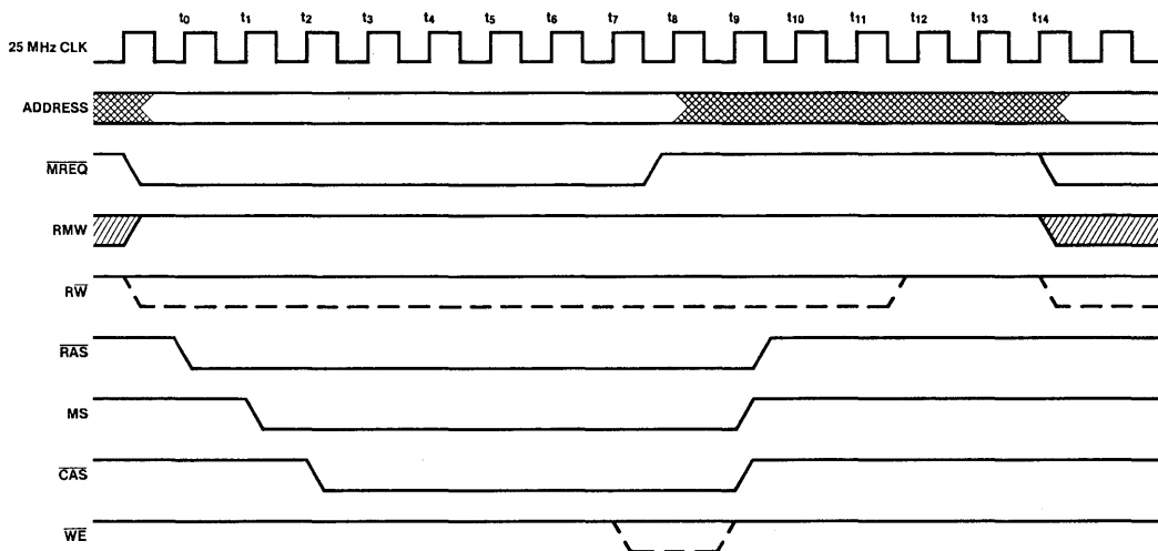
Figure 5. Read-Modify-Write Cycle
