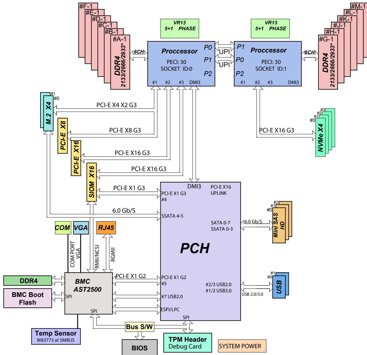
Figure 1-3. System Block Diagram for the X11DPFF-SN Motherboard
