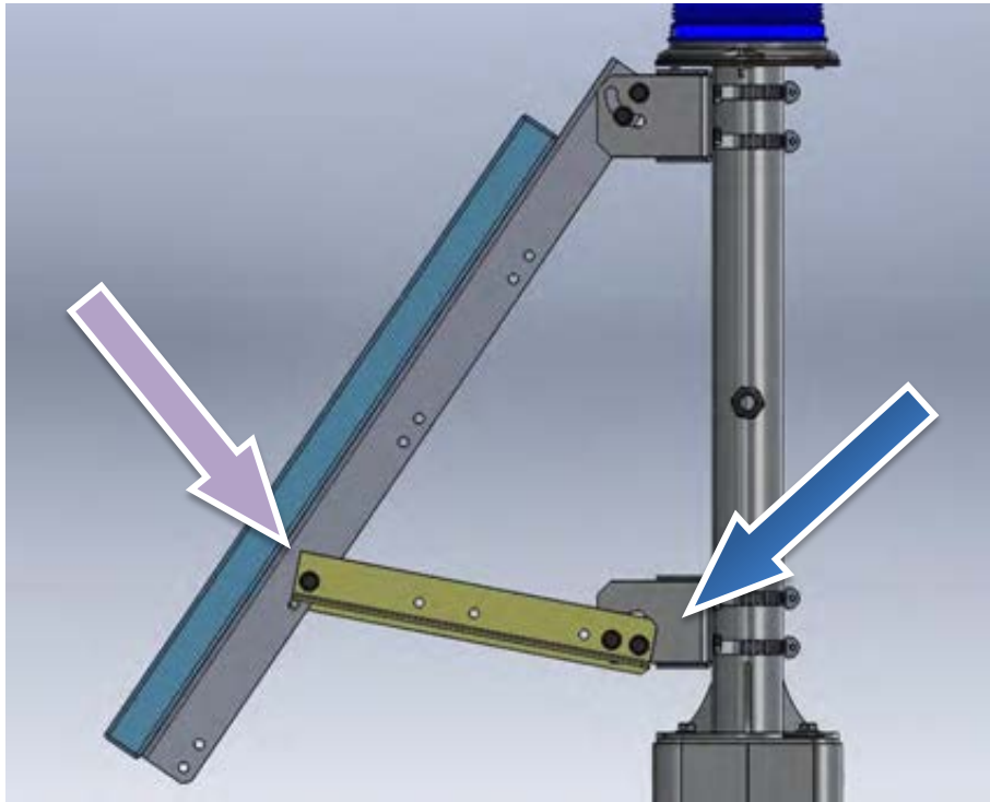
Figure 21. Support rail installation for a solar panel with a tilt angle of 55°
