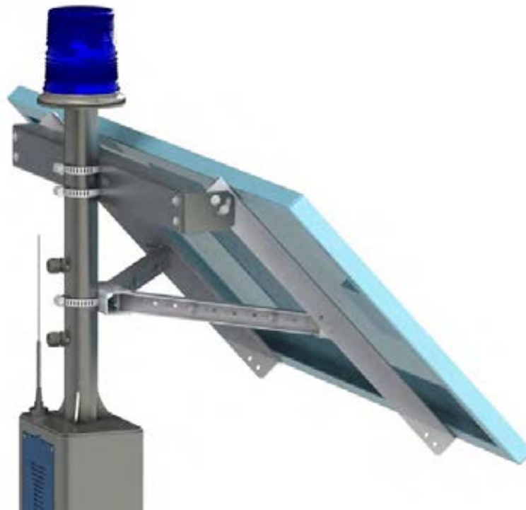
Figure 14. Assembled view of SLR-80-84 (shown on ETP-MTE-WP )
