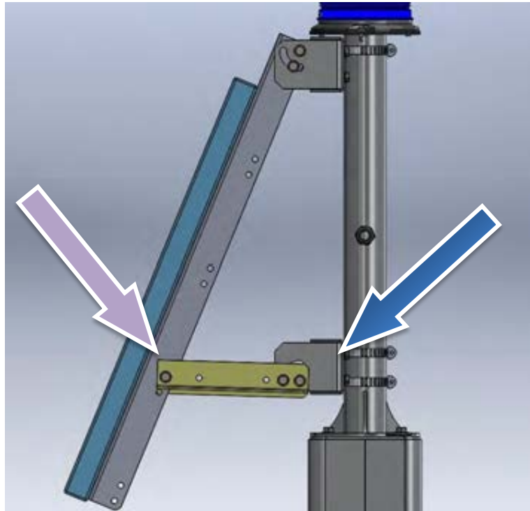
Figure 23. Support rail installation for a solar panel with a tilt angle of 65°
