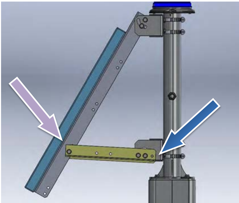
Figure 22. Support rail installation for a solar panel with a tilt angle of 60°
