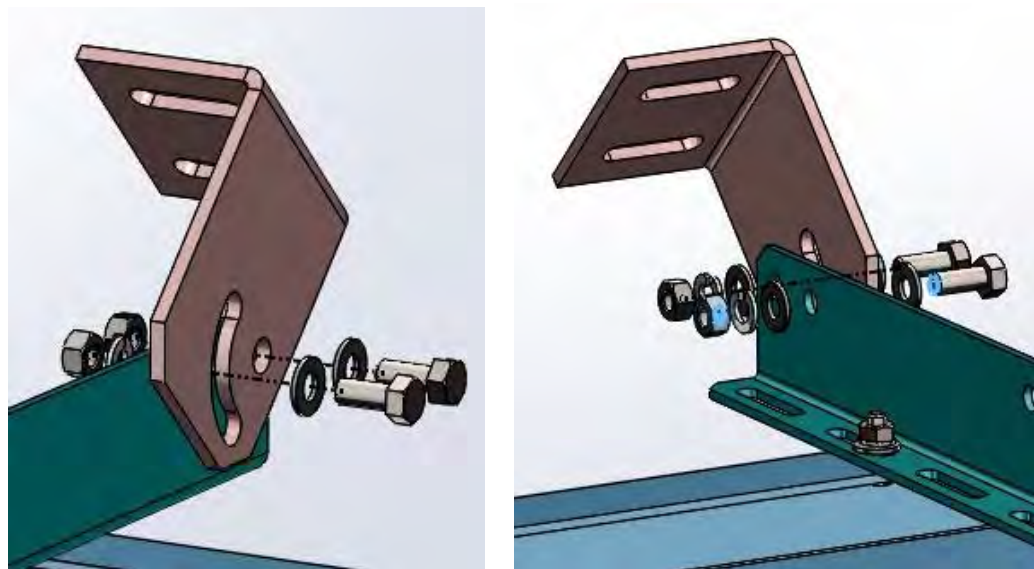
Figure 6. Exploded view of right clip attached to the right mounting rail
