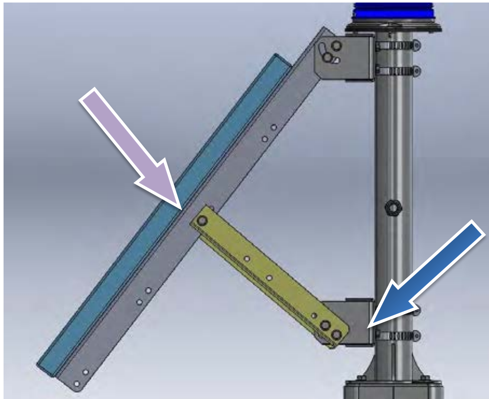
Figure 20. Support rail installation for a solar panel with a tilt angle of 50°
