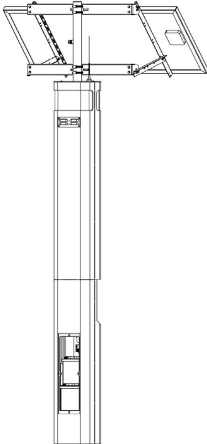
Figure 32. ETP-MT/R OP SOLAR with access panel removed, assembly overview (SLR-120-84)
