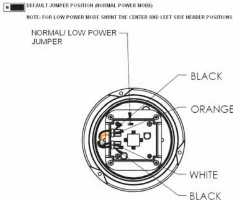
Figure 30. Normal / Low power mode jumper inside LED Blue Light
