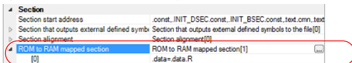
Figure 2.37 [ROM to RAM mapped section] Property
