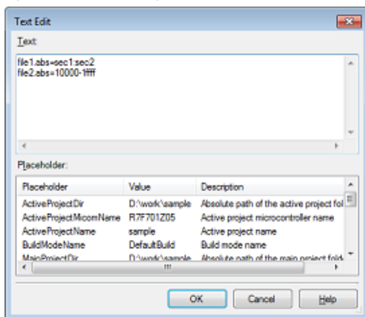
Figure 2.57 Text Edit Dialog Box
