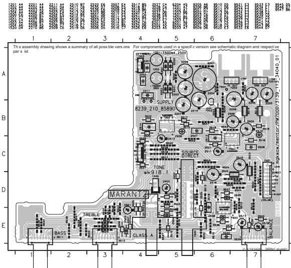
FRONT BOARD
