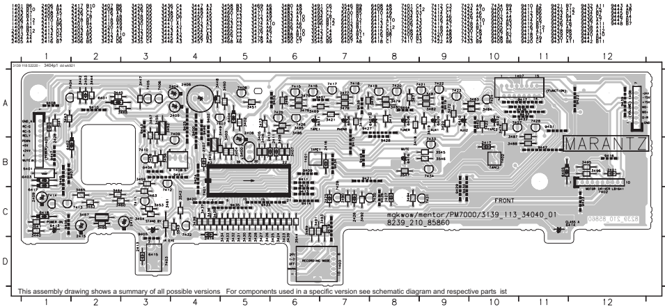
FRONT BOARD
