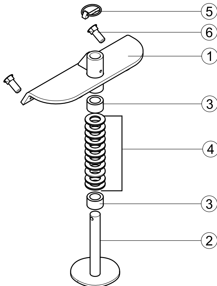
SKID SHOE 35 Series Rear Blade
