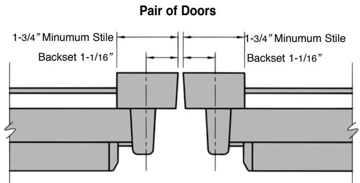
Two Concealed Vertical Rod Devices
