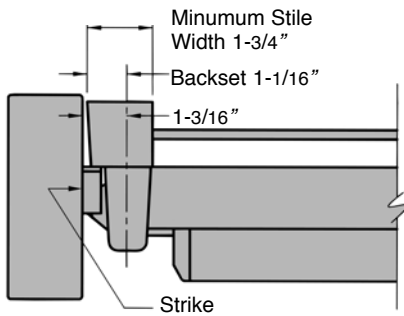
Rim Device with S988 Strike
