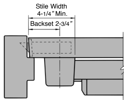
Mortise Device
