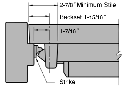
Rim Device with S300 or S301 Strikes
