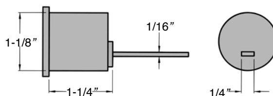
Rim Cylinder - 1E72 x Finish
