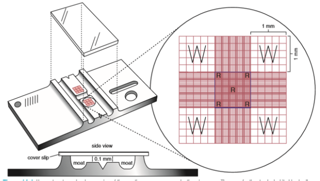
Figure 1: Neubauer glass hemocytometer
