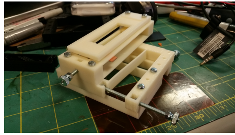
Figure 4: 3D-printed XYZ stage with adjustment screws and a hemocytometer slot
