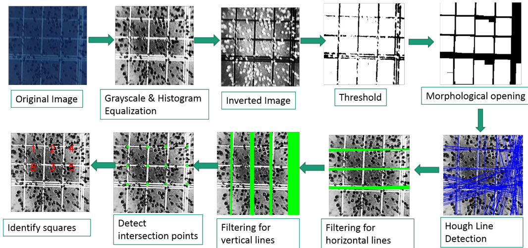
Figure 6: Square detection
