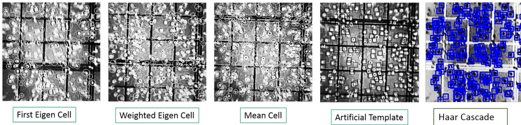
Figure 5: Cell detection
