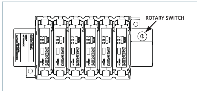
Figure 10: Six Pole Meter Module Rack with 10 Position Rotary Switch
