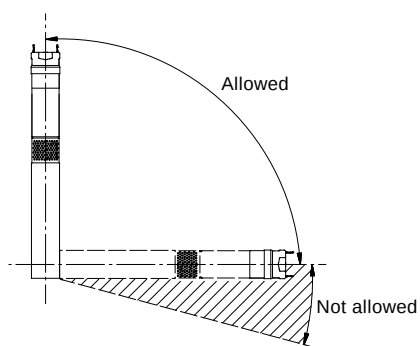
Fig. 13 SQE installation
