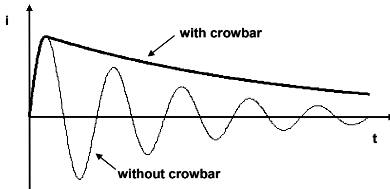
Fig. 21 - Principle of an impulse current generator with crowbar devices
