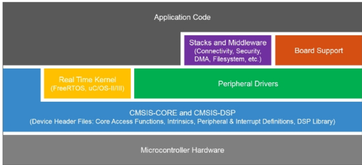
Figure 1. KSDK layers
