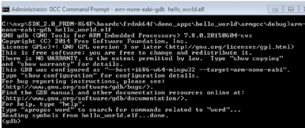
Figure 50. Run arm-none-eabi-gdb
