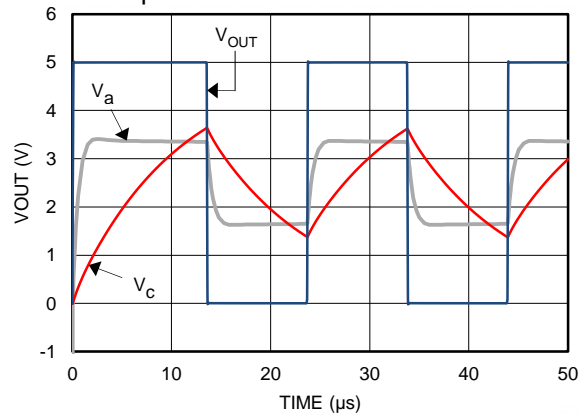
Figure 25. Square-Wave Oscillator Output Waveform
