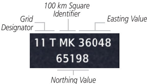
Figure 15-46 MGRS Position Format Detail
