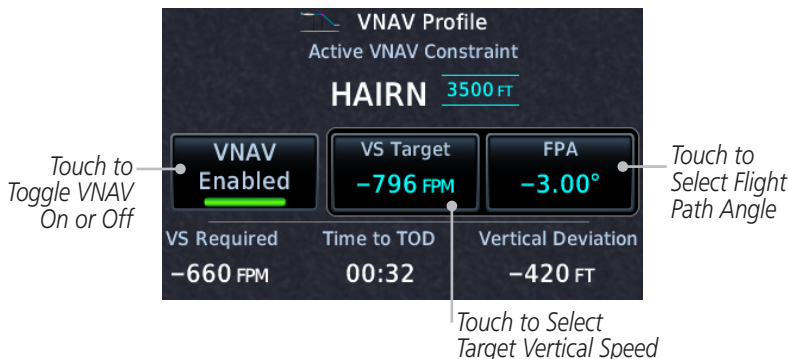
Figure 4-46 VNAV Profile Page
