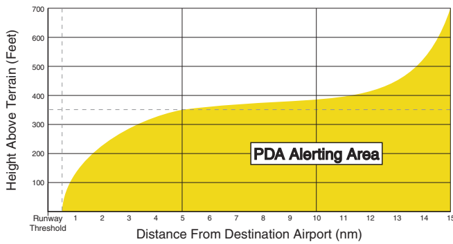
Figure 10-10 PDA Alerting Threshold
