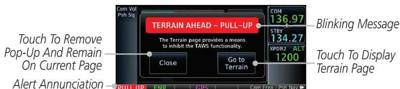
Figure 10-9 Terrain Alert Pop-Up
