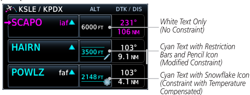
Figure 4-47 Waypoint Altitude Constraints
