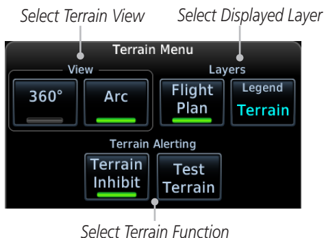
Figure 10-7 Terrain Menu
