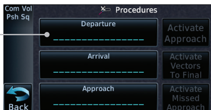
Figure 6-2 Select Departure
