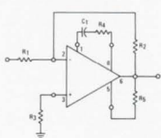
FIGURE 1 - TEST CIRCUIT
