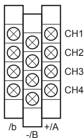
4 Pen Screw Type
