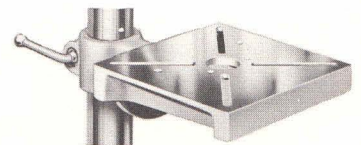
Well ribbed table tilts to 45° either direction. Has index pin to assure angular setting. Slots in table and ledge on each side for convenient clamping of work.
