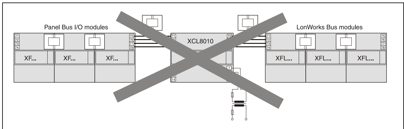
Fig. 24. Mixed bus system – incorrect wiring
