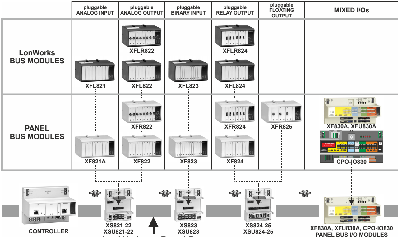
Fig. 3. Overview of Honeywell I/O modules
