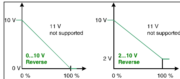
Fig. 75. Analog output control levels – reverse actuator
