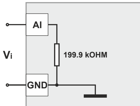
Fig. 31. Analog input high impedance (input circuit for voltage input for active sensors)
