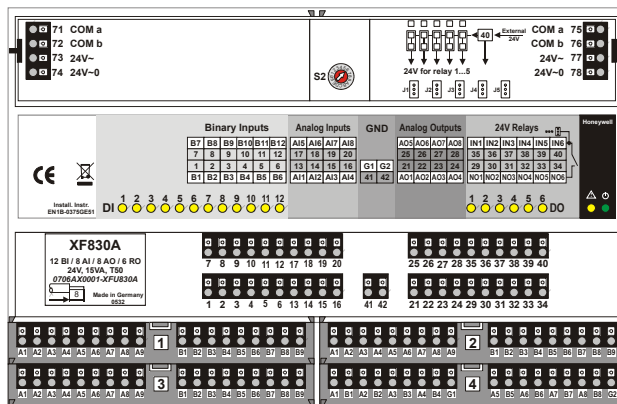
Fig. 56. XF830A Mixed I/O Module (shown with aux. terminal packages)
