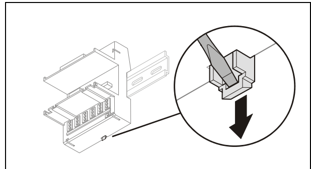
Fig. 10. Releasing latch
