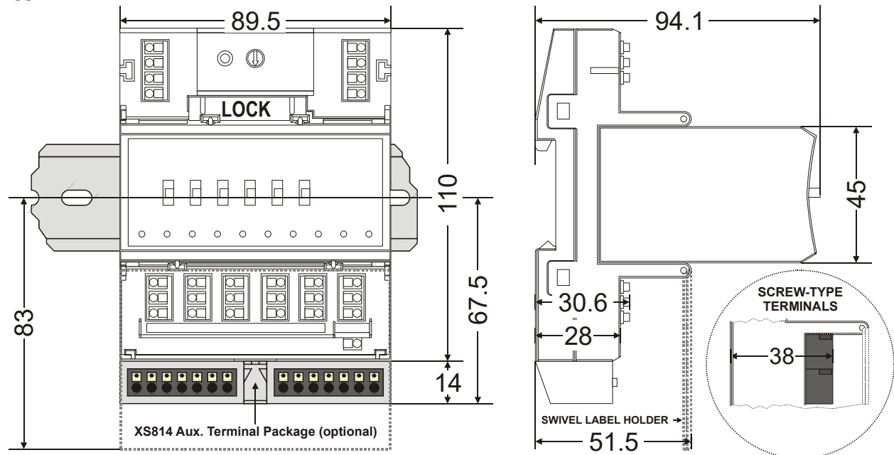
Fig. 4. Pluggable I/O modules (shown with manual overrides), including XS814 Aux. Terminal Package, dimensions (in mm)
