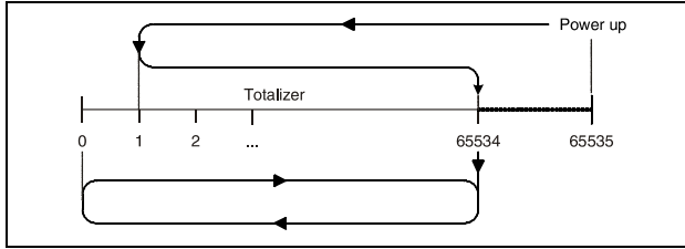
Fig. 77. Totalizer
