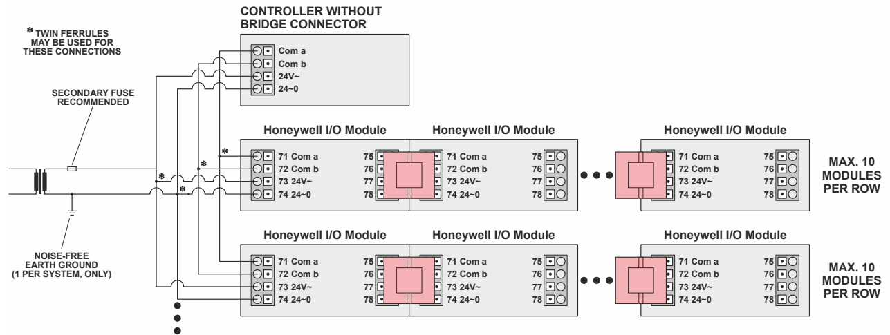
Fig. 22. Wiring controllers not supporting bridge connectors
