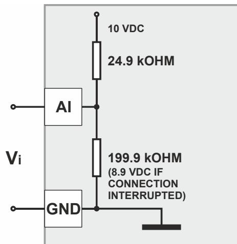
Fig. 60. Analog input impedance setpoint (input circuit for NTC10k \Omega , NTC20k \Omega , wall module setpoint)
