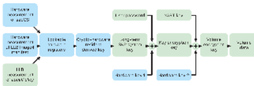
The Sealed Key Protection process in a Mac with Apple silicon.
