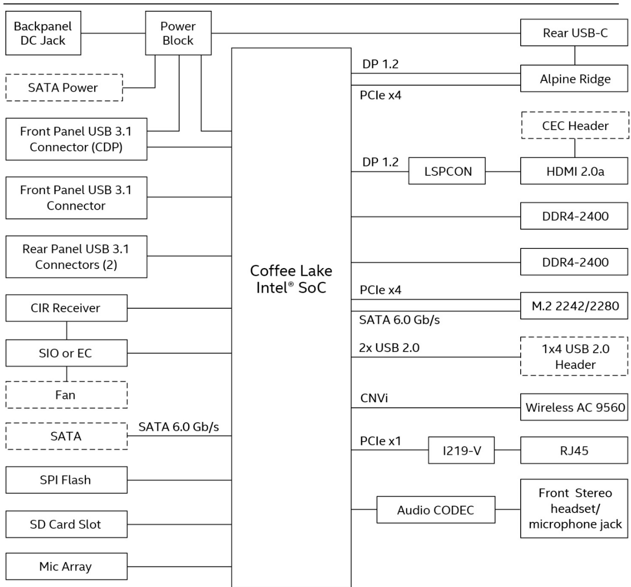
Figure 3. Block Diagram
