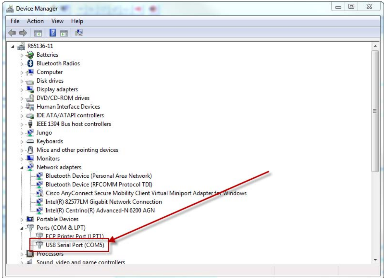
Figure 6. Device Manager
