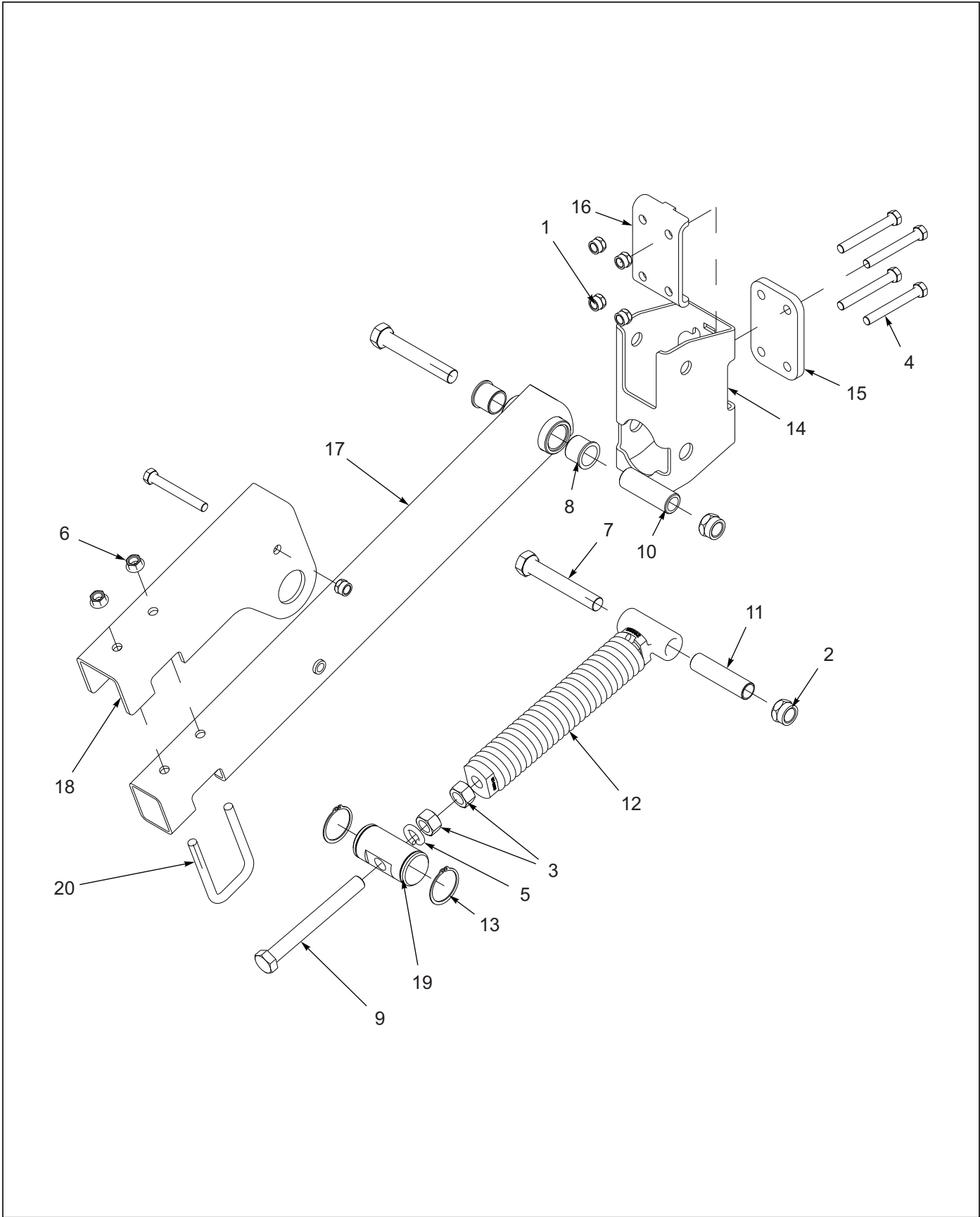
Figure 1-19: 4 Row Coil Tine Harrow Arm Assembly
