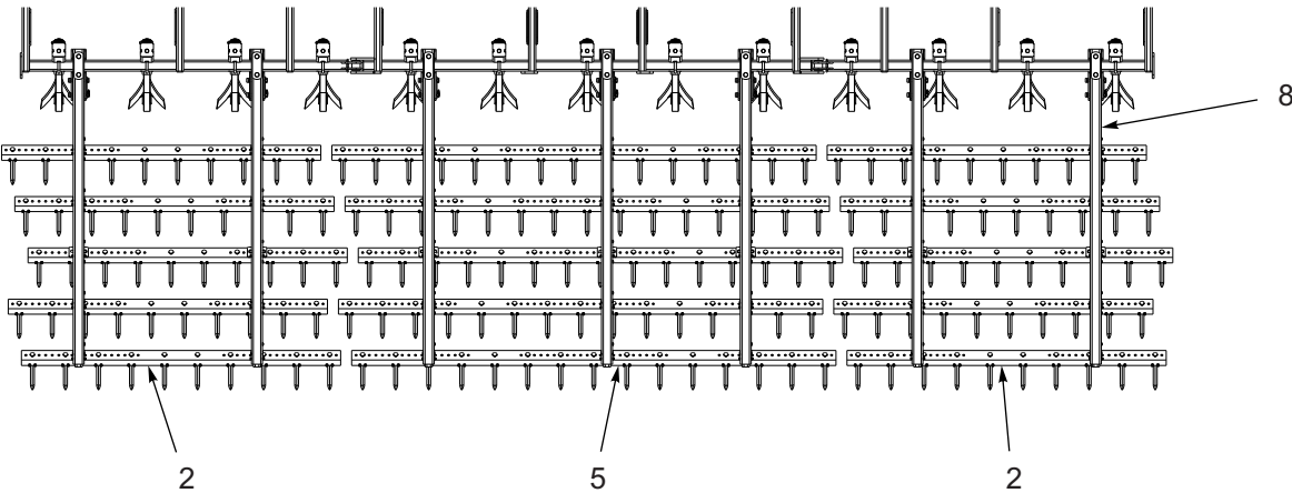
MODEL 9630-24 (P/N 187527)
