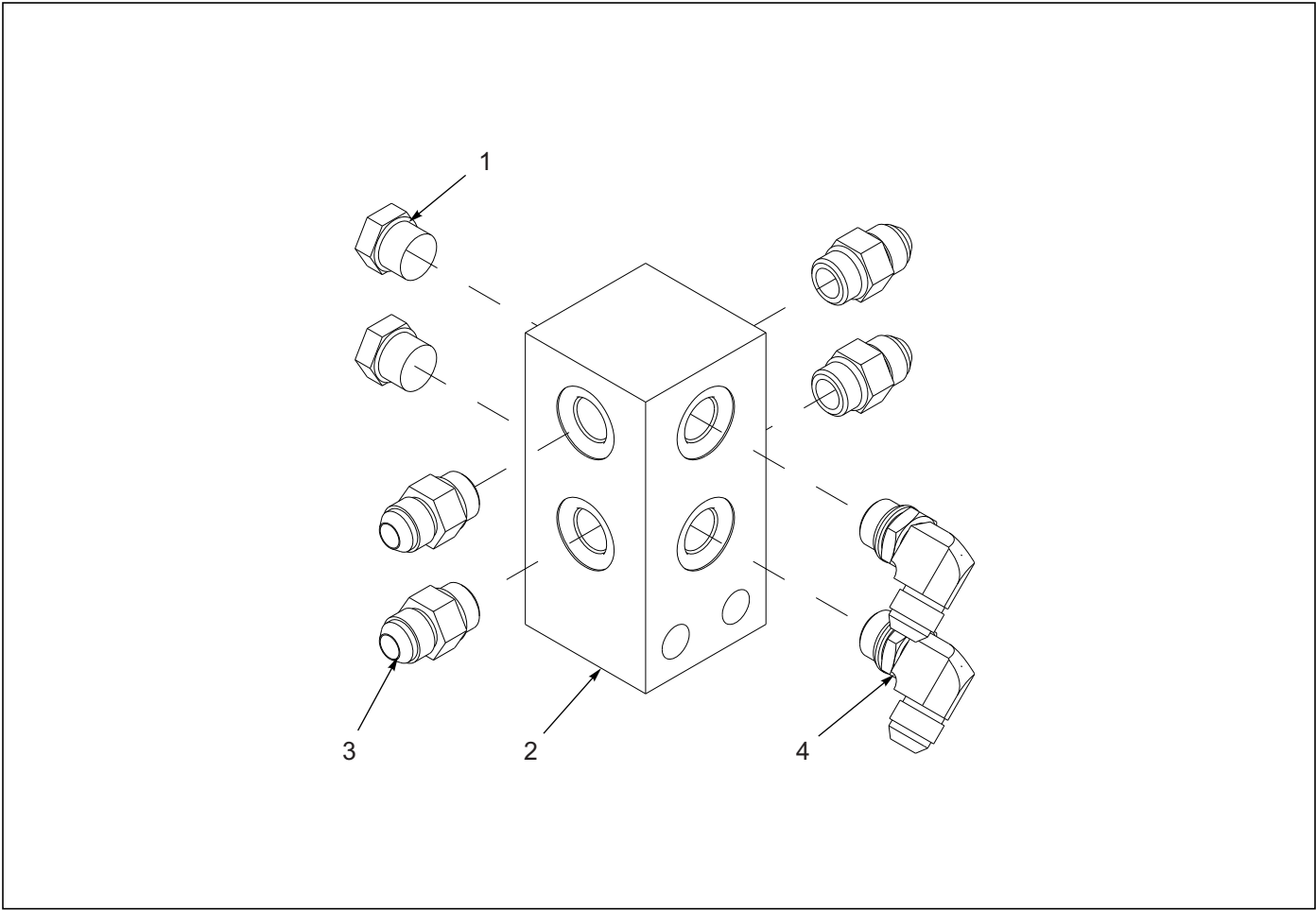
Figure 1-58: Manifold Assembly, Lift
