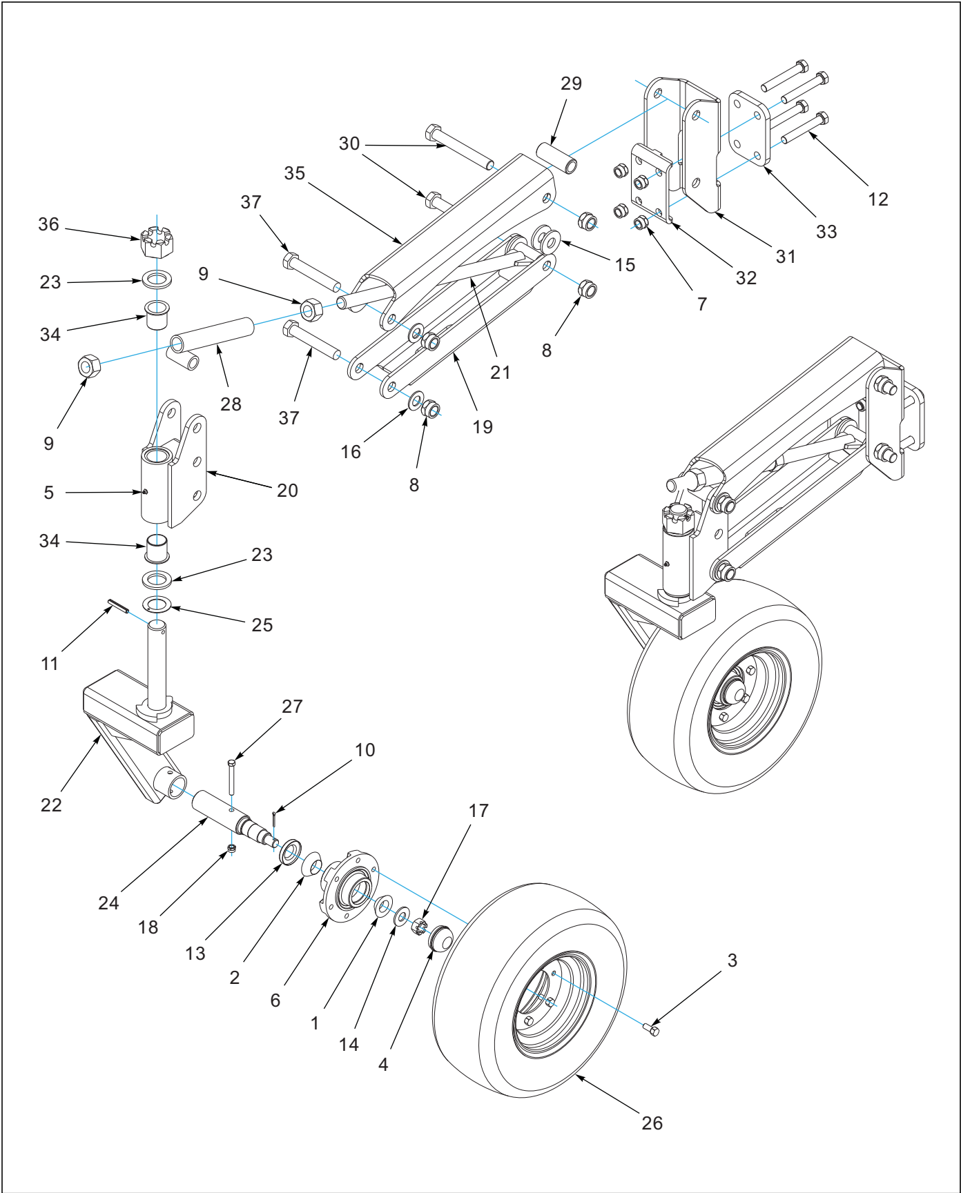
Figure 1-9: Front Gauge Wheel Assembly
