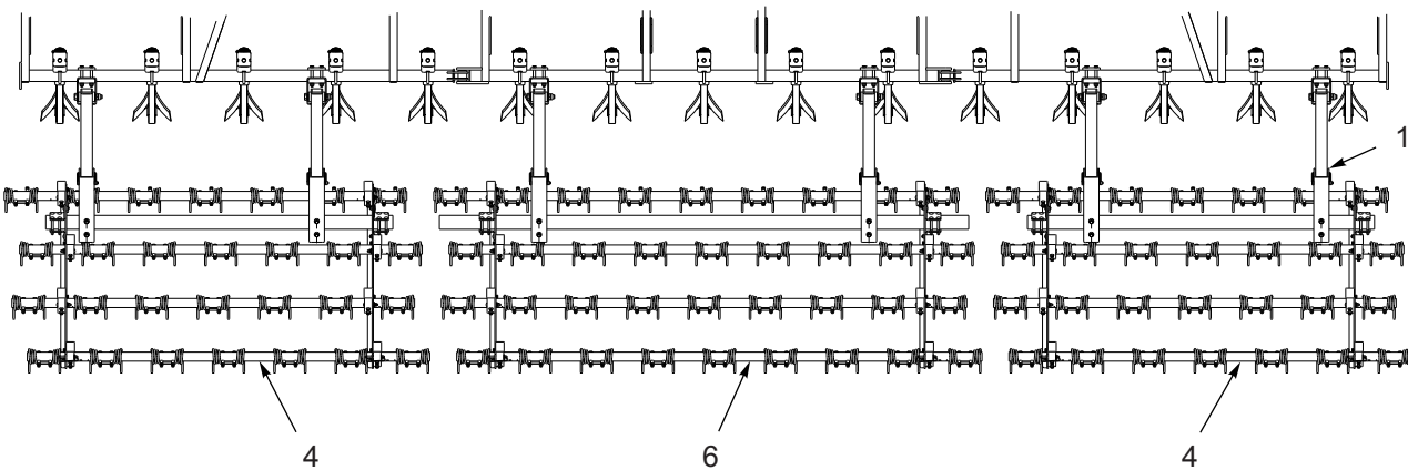
MODEL 9630-28 (P/N 166303)
