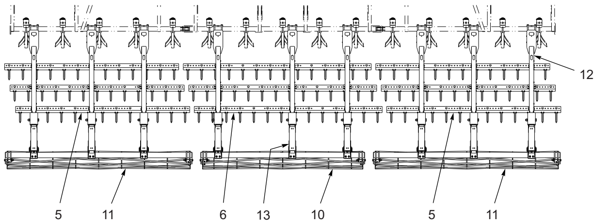
MODEL 9630-28 (P/N 187557)
