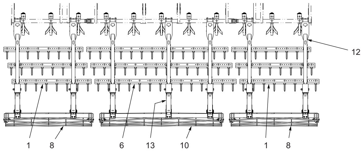
MODEL 9630-20 (P/N 187555)
