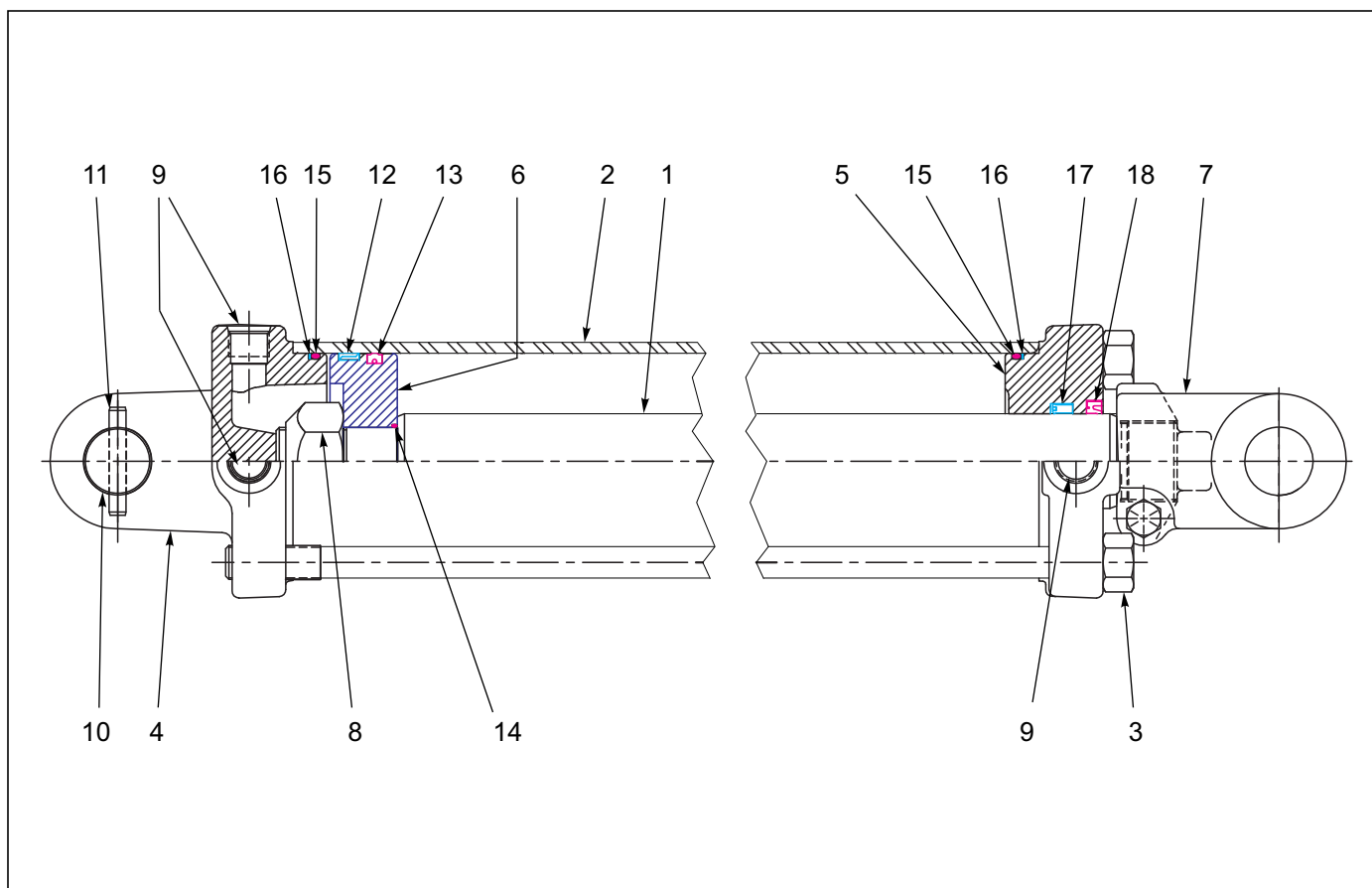
Figure 1-62: Cylinder - 4" X 30" (1-1/2" Dia Rod)
