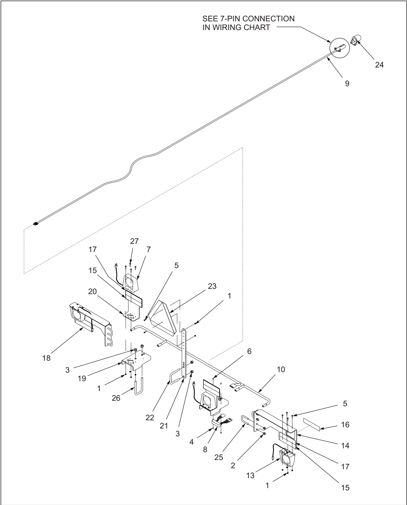
Figure 1-43: Electrical Assembly (Prior to August, 2013) (1 of 2)
