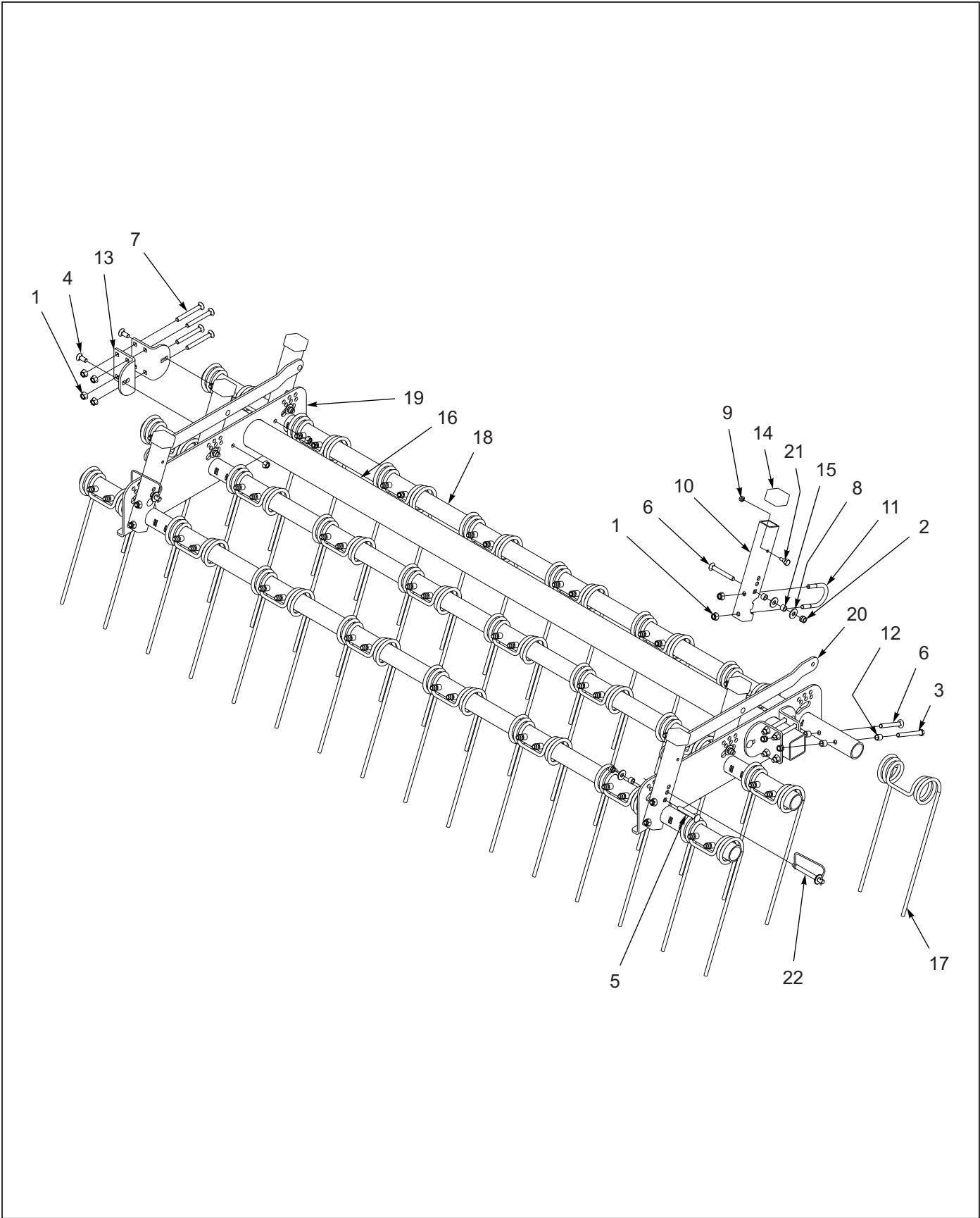
Figure 1-25: 3 Row Coil Tine Harrow Assembly
