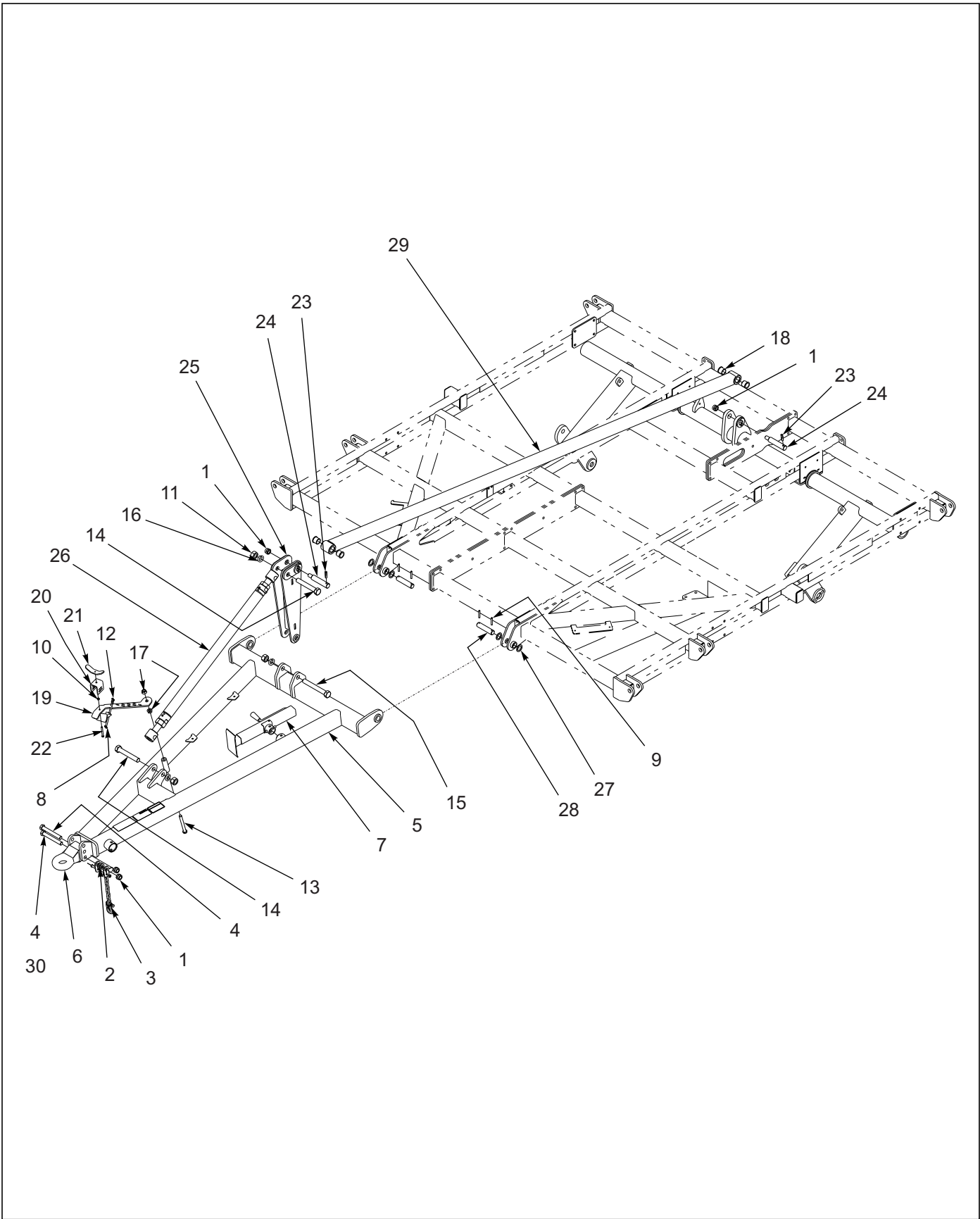
Figure 1-10: Hitch and Leveling Linkage Assembly
