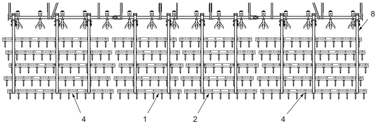
MODEL 9630-30 (P/N 187529)
