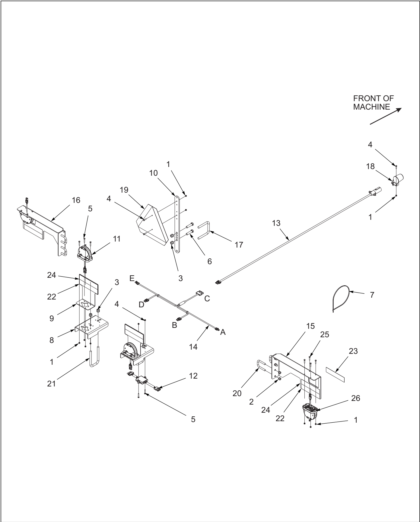
Figure 1-45: Electrical Assembly (After August, 2013) (1 of 2)
