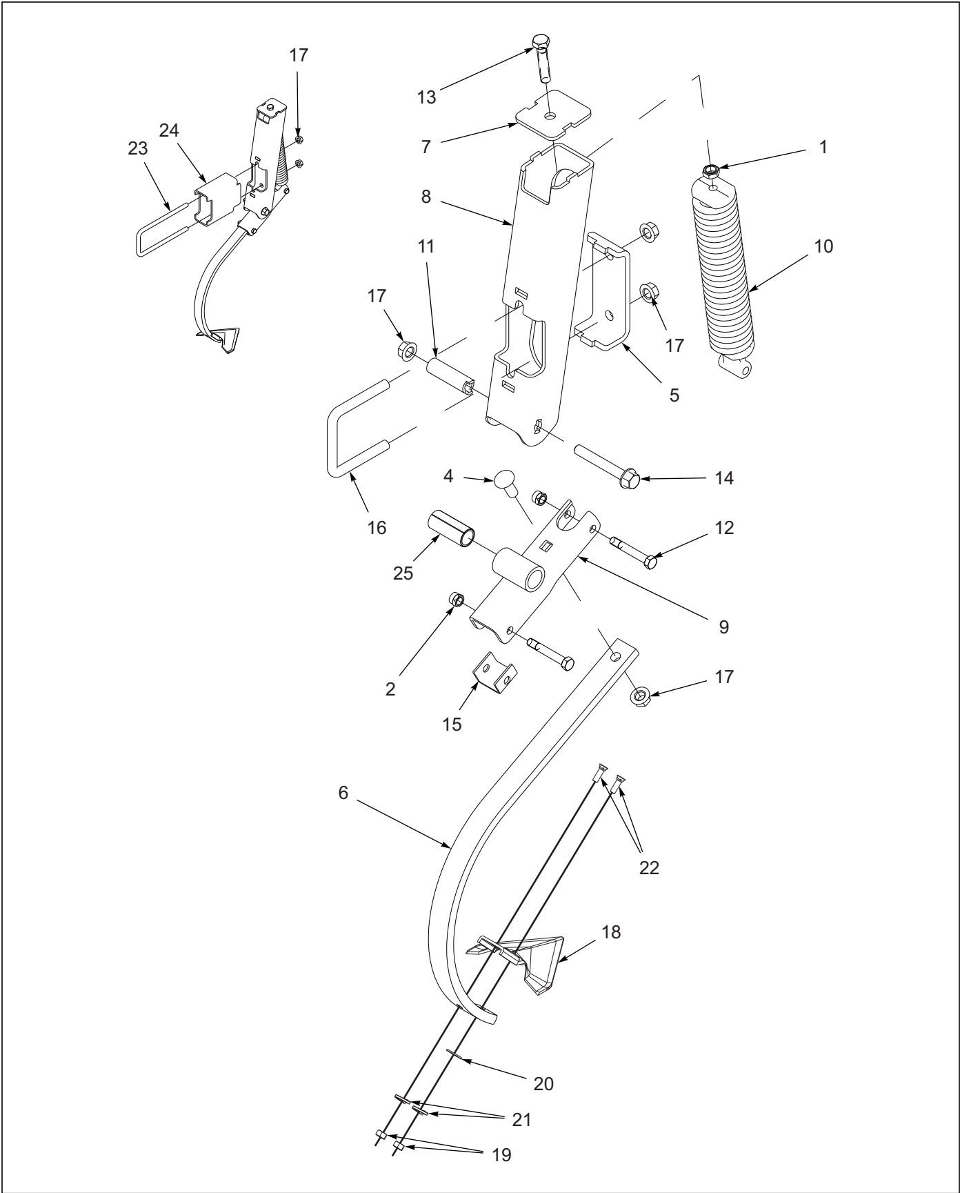
Figure 1-13: Spring Shank Assembly (Prior to 08/23/2012)
