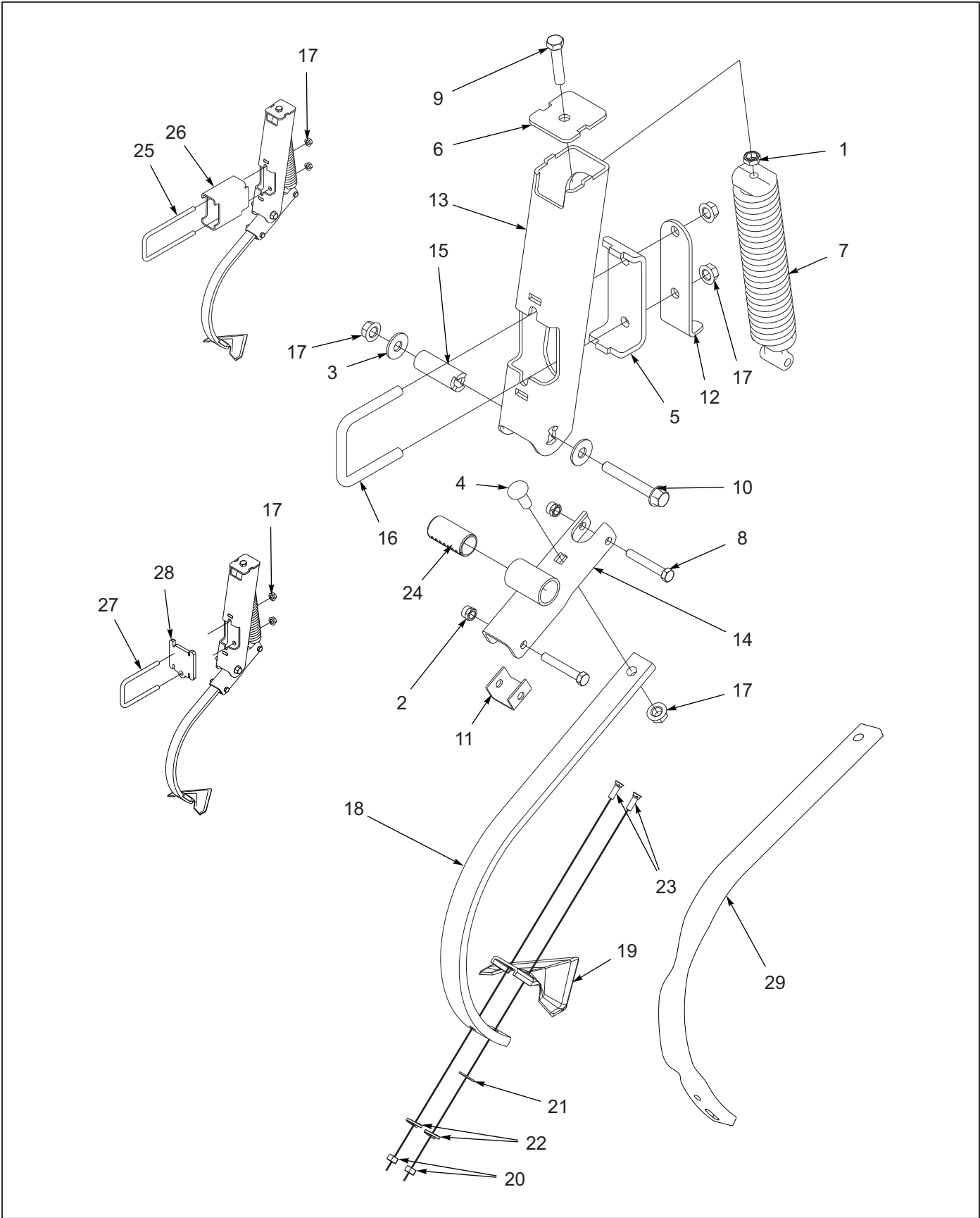
Figure 1-14: Spring Shank Assembly (After 08/23/2012)
