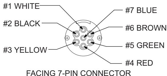
Figure 1-44: Electrical Assembly (Prior to August, 2013) (2 of 2)
