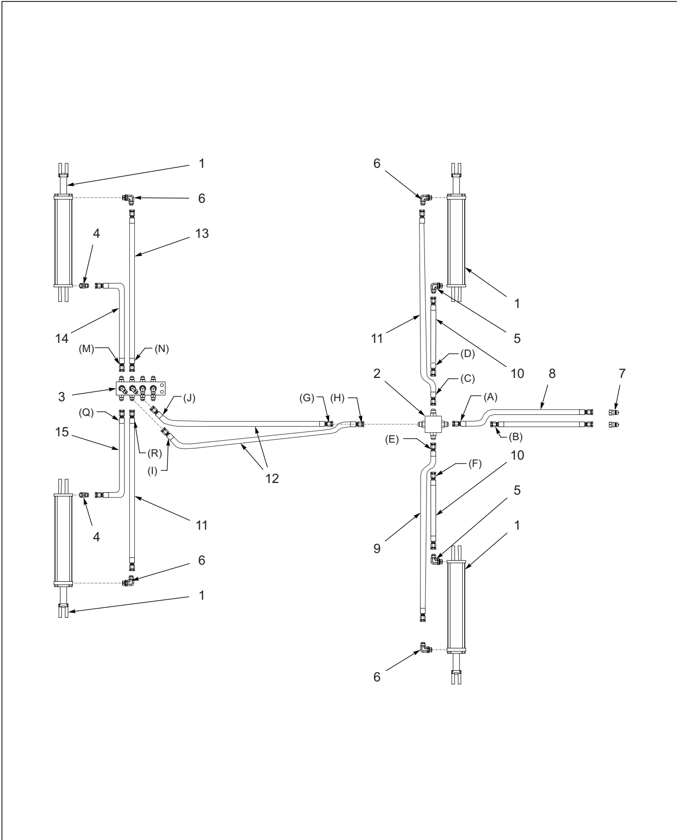
Figure 1-52: Fold Hydraulic Assembly (9630-28 Model)
