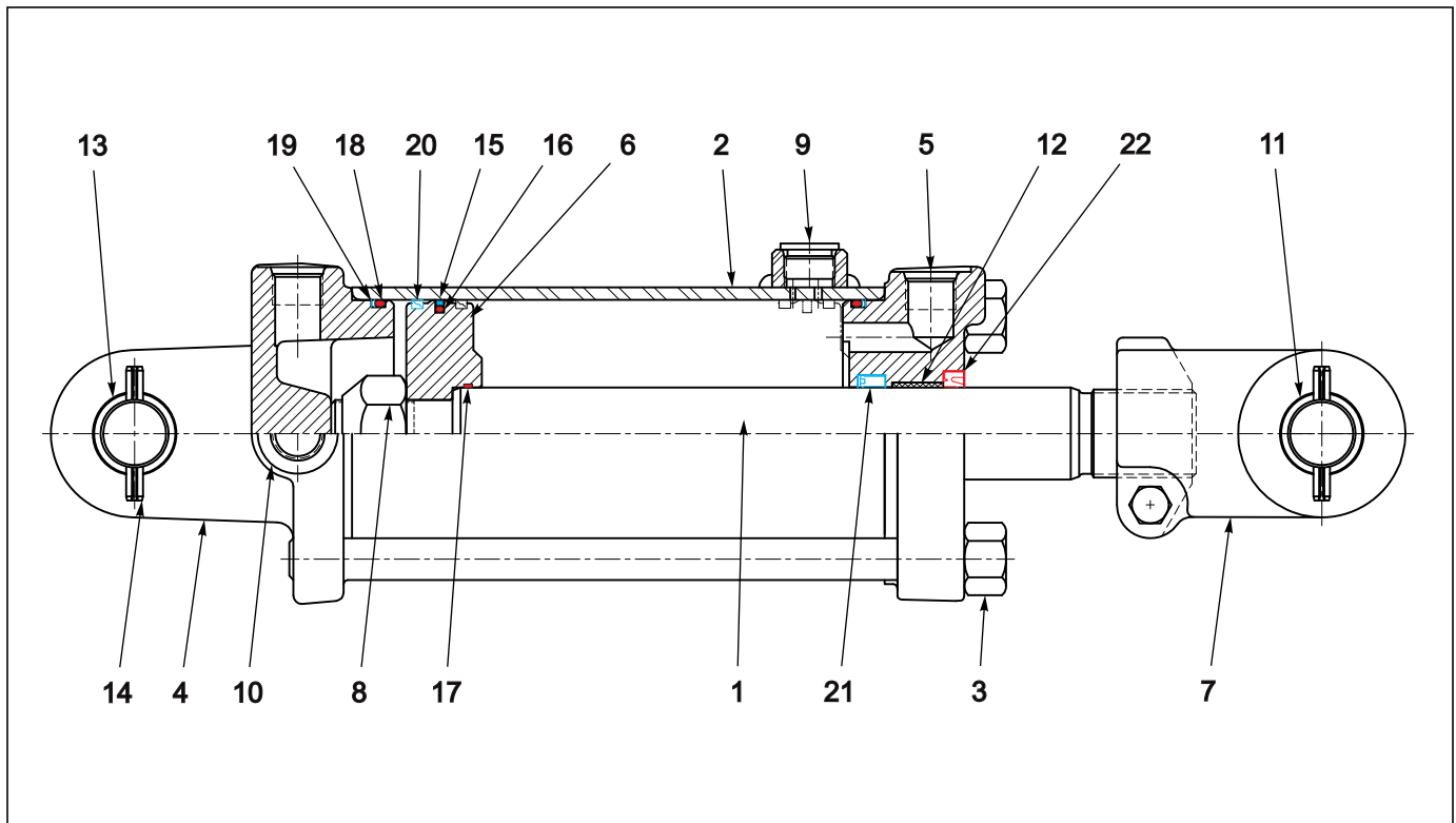
Figure 1-61: Cylinder - Rephase Assembly 4 X 10 (1" Clevis Pins)
