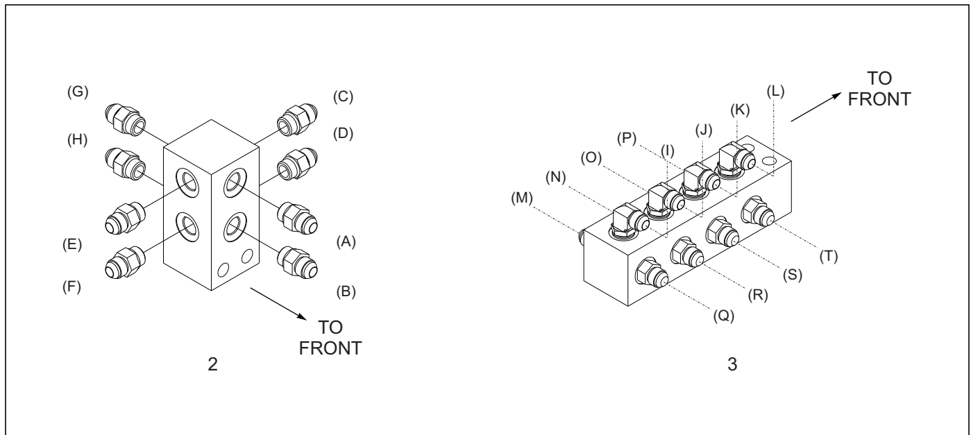
Figure 1-53: Fold Hydraulic Assembly (9630-28 Model)
