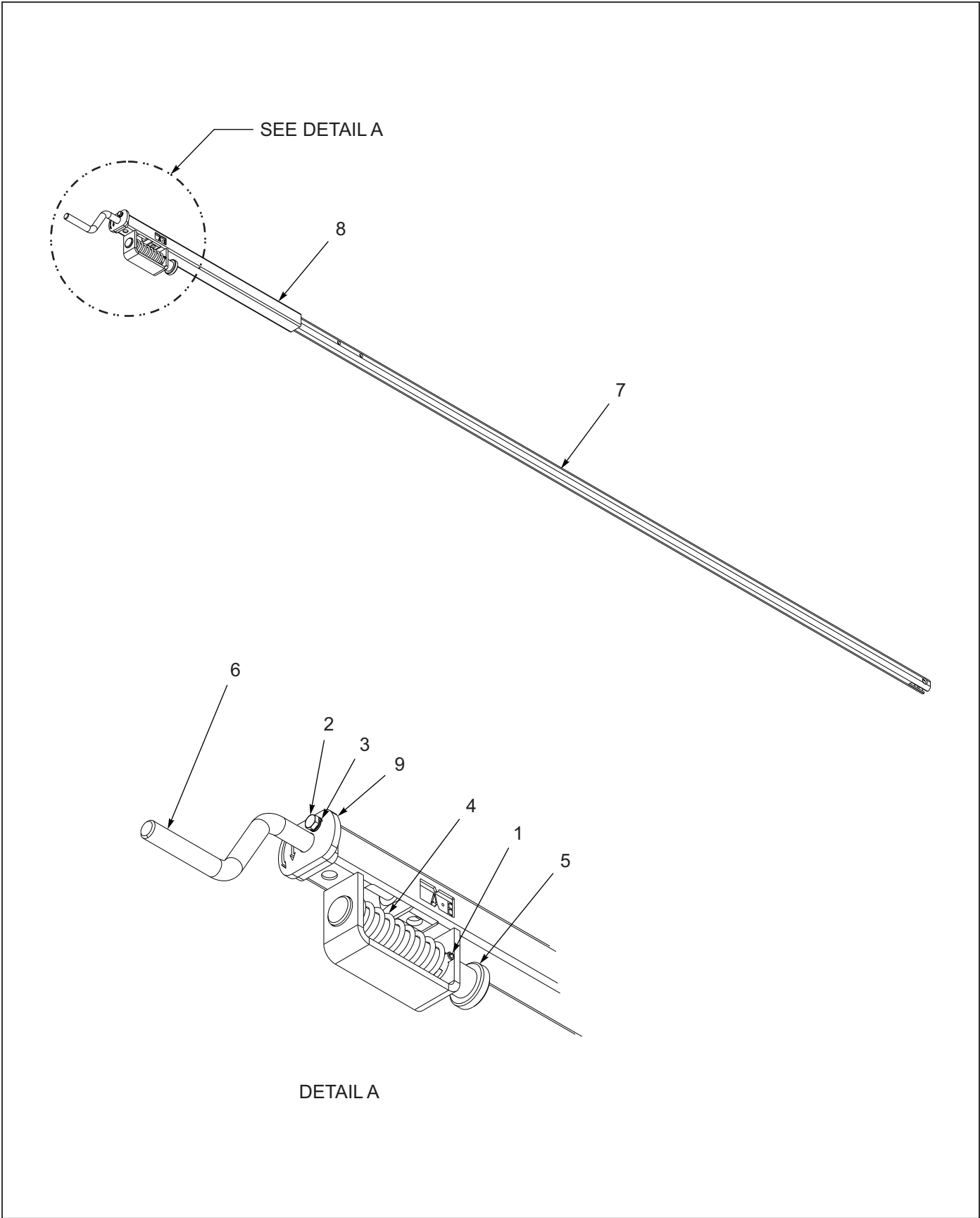
Figure 1-8: Depth Stop Tube Assembly
