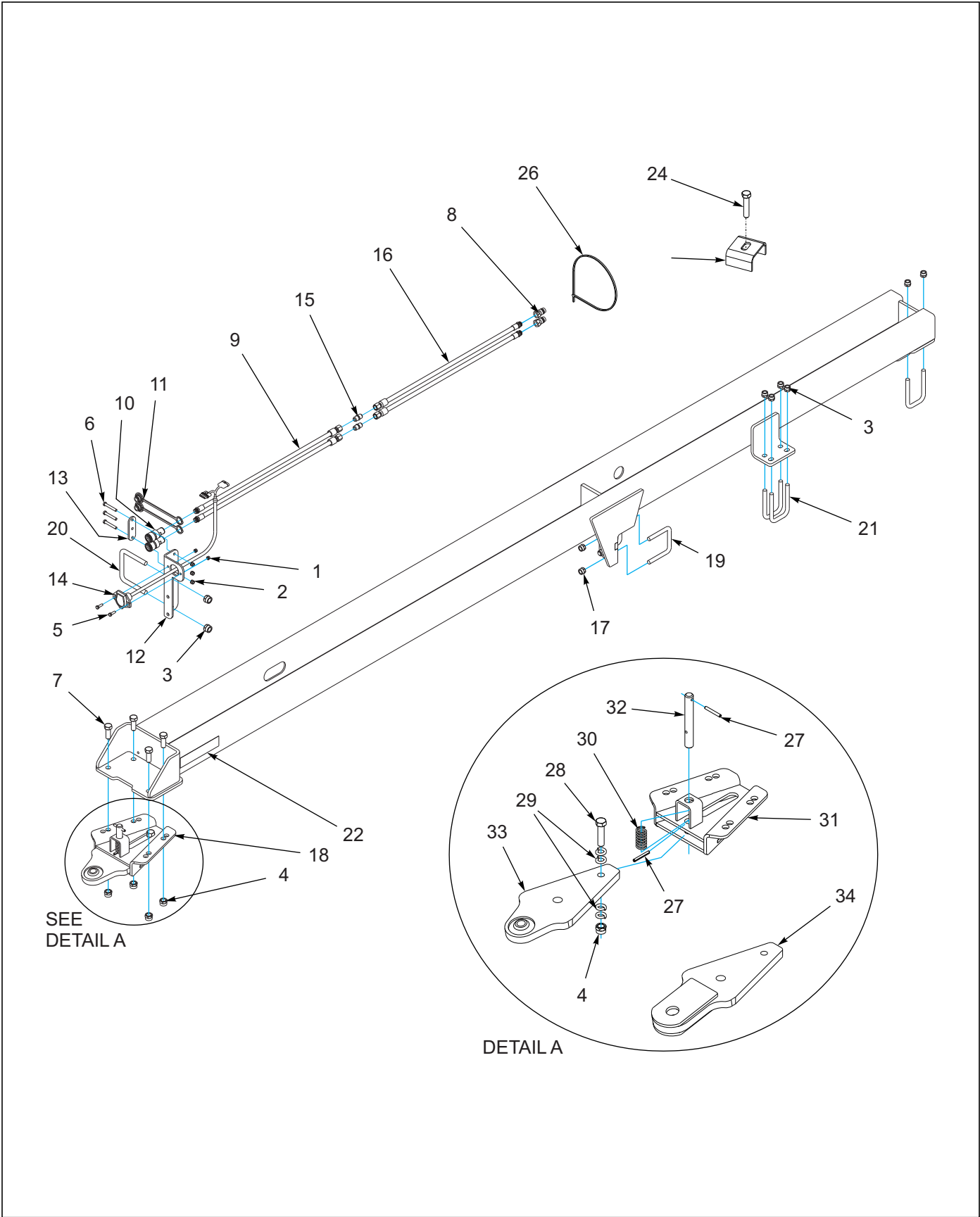
Figure 1-41: Rear Tow Hitch Assembly (20' - 28' Models)
