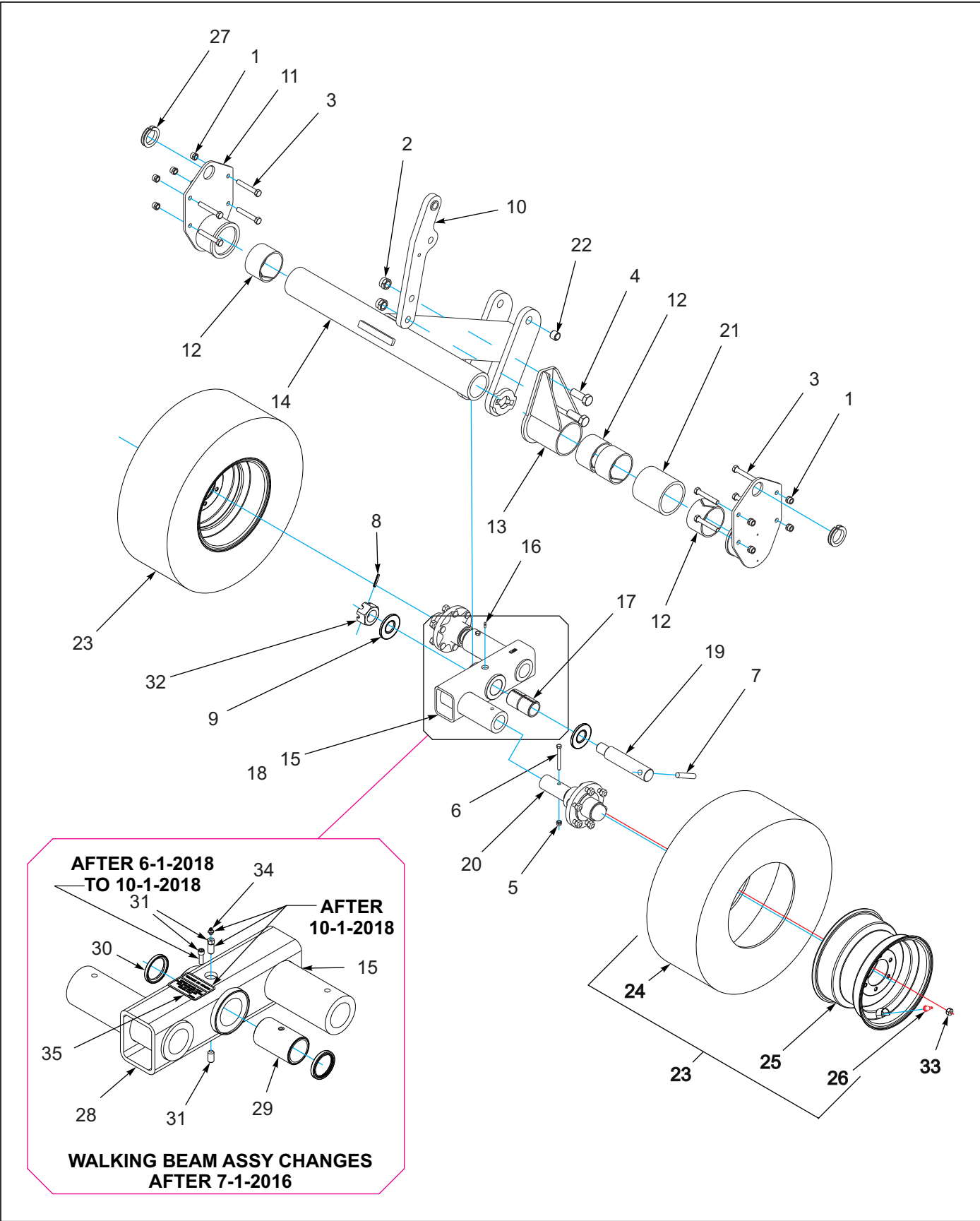
Figure 1-6: Wing Lift Assembly
