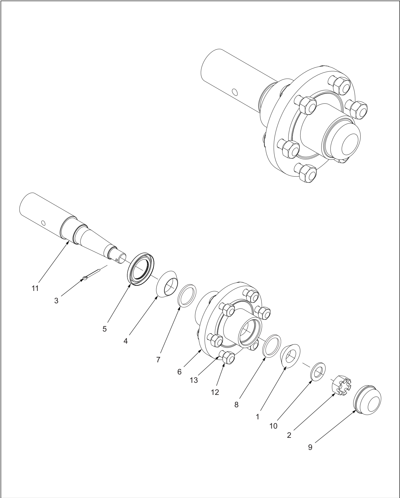
Figure 1-7: Hub and Spindle Assembly, 6-Bolt
