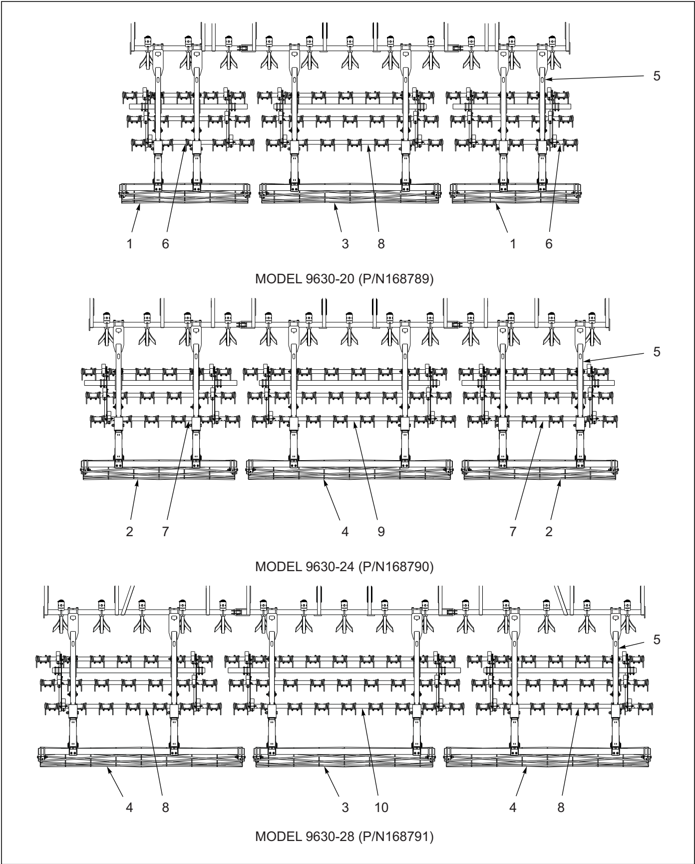
Figure 1-21: 3 Row Coil Tine and Reel Harrow Assembly (1 of 3)
