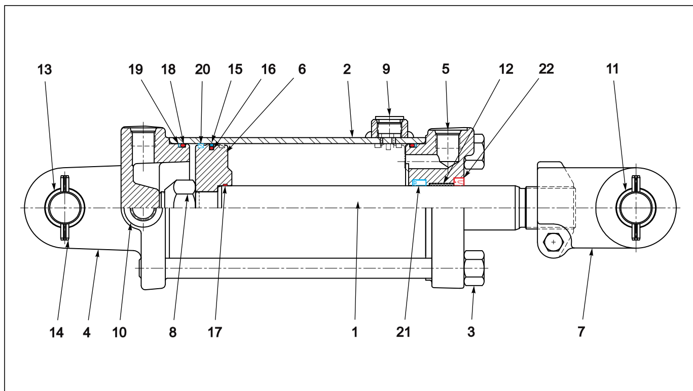
Figure 1-60: Cylinder - Rephase Assembly 3-3/4 X 10 (1" Clevis Pins)
