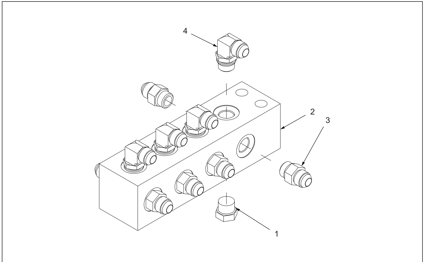
Figure 1-57: Manifold Assembly, Lift/Fold
