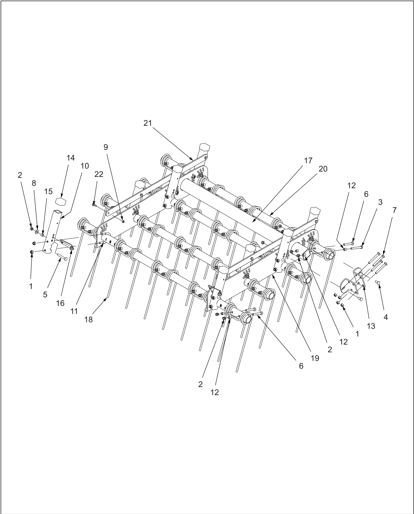
Figure 1-20: 4 Row Coil Tine Harrow Assembly
