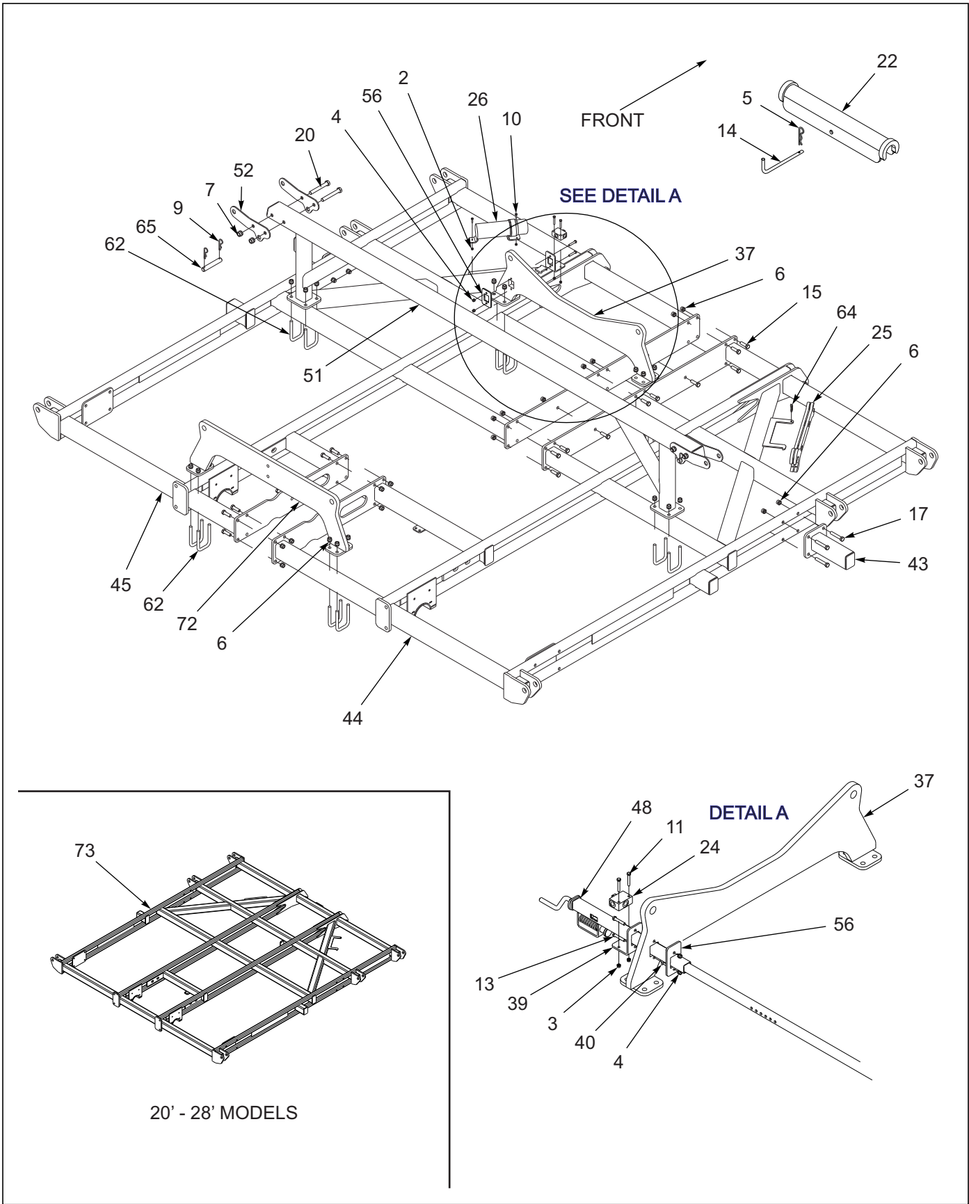
Figure 1-2: Center Frame and Lift Assembly (1 of 2)
