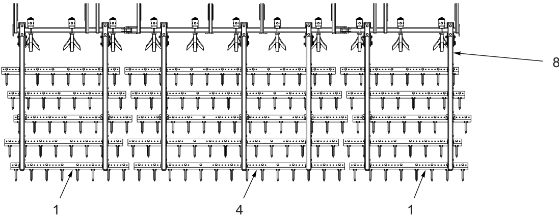
MODEL 9630-20 (P/N 187526)
