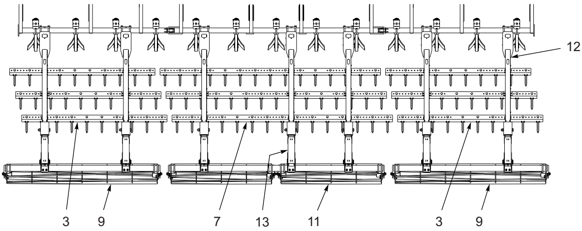
MODEL 9630-24 (P/N 203079)
