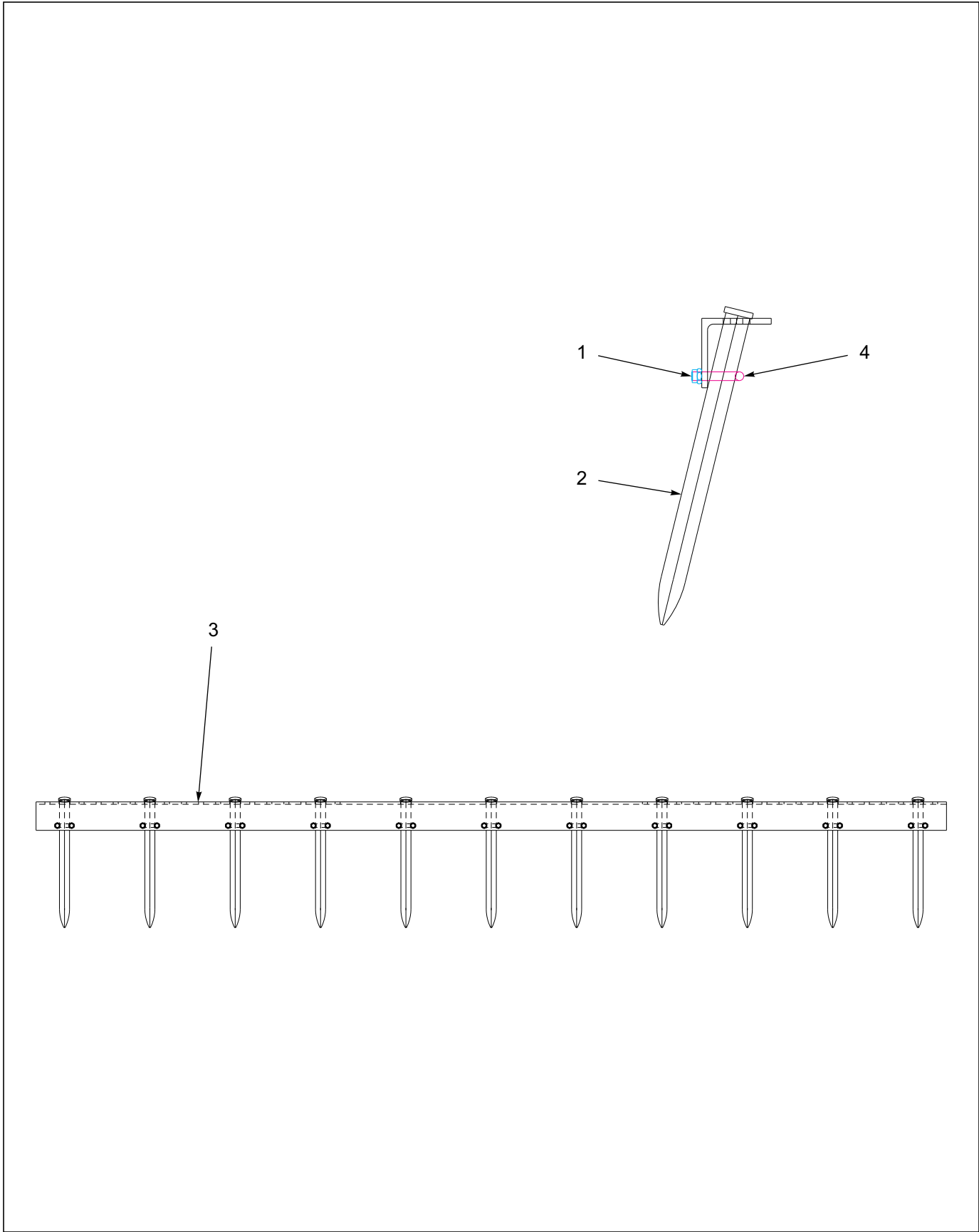
Figure 1-38: Spike Bar Assembly, 9 SP
