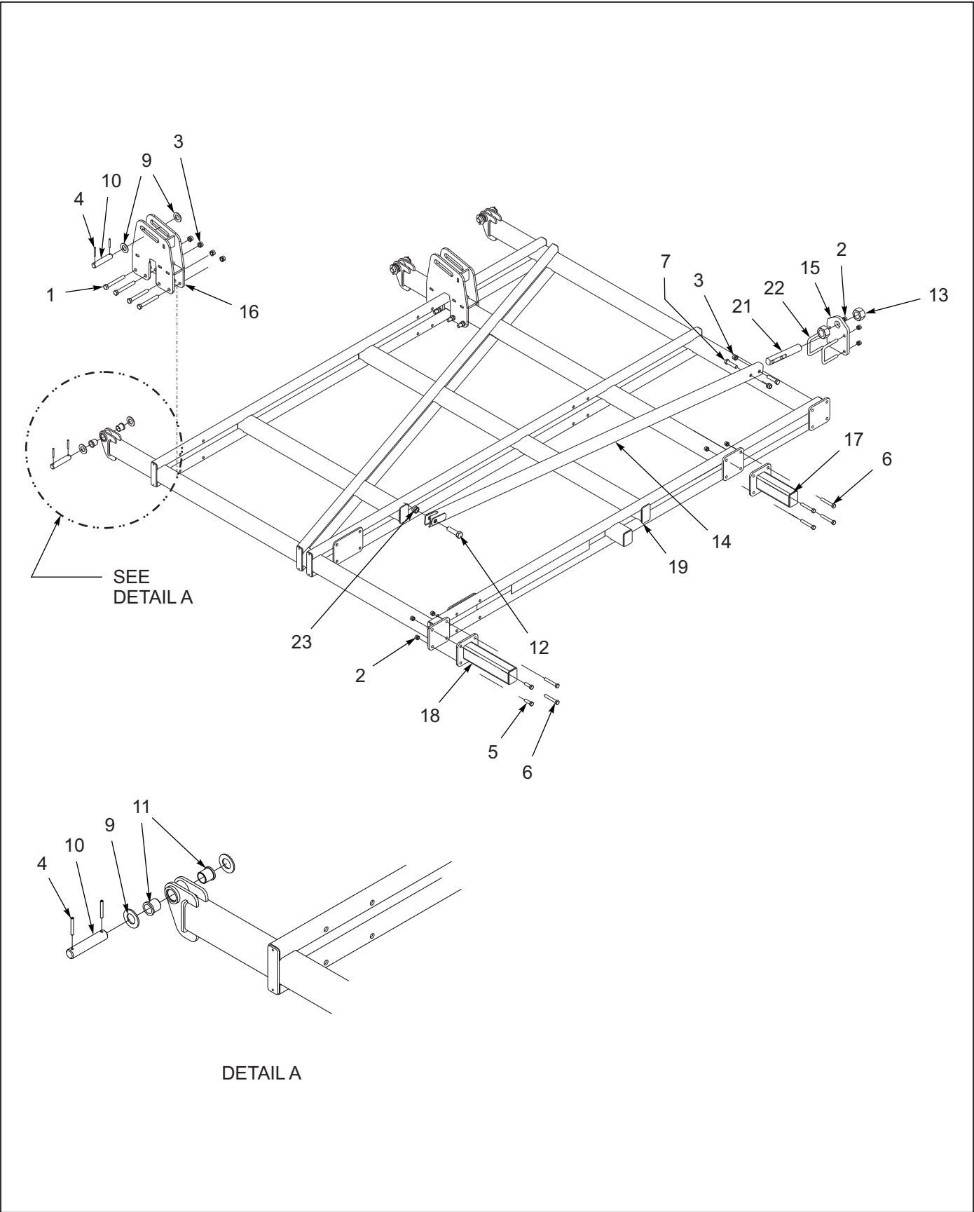
Figure 1-5: Wing Assembly
