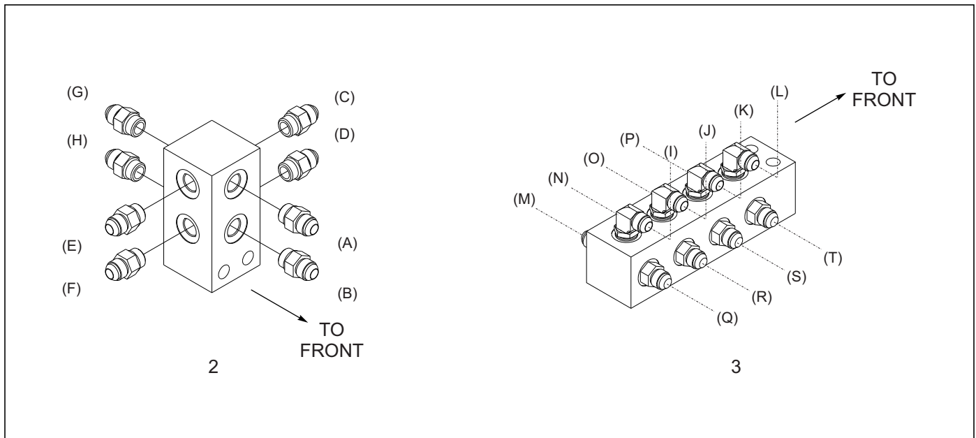
Figure 1-55: Fold Hydraulic Assembly (9630-30 &amp; 9630-34 Models)
