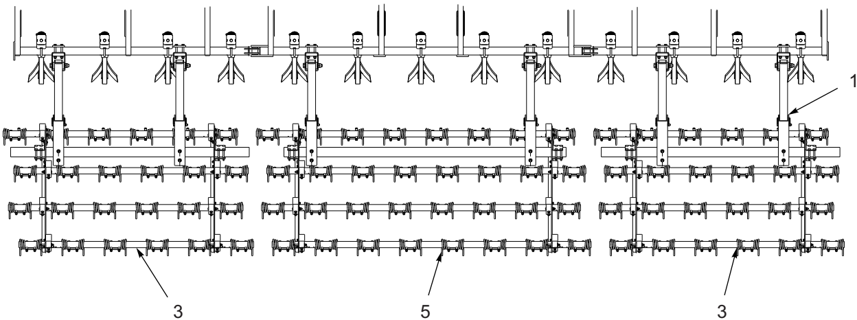
MODEL 9630-24 (P/N 166302)
