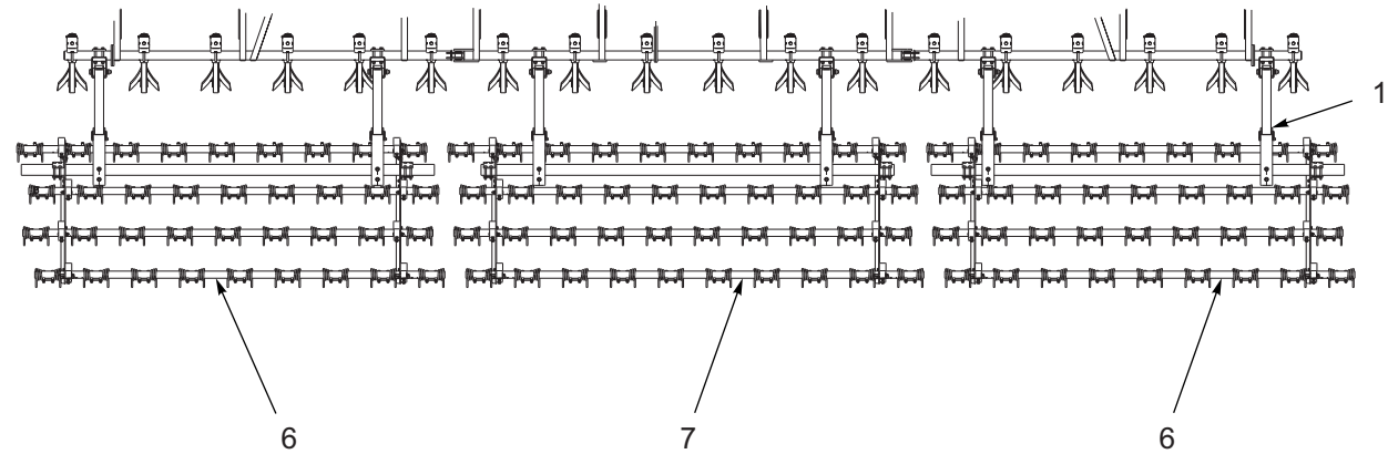
MODEL 9630-34 (P/N 166305)
