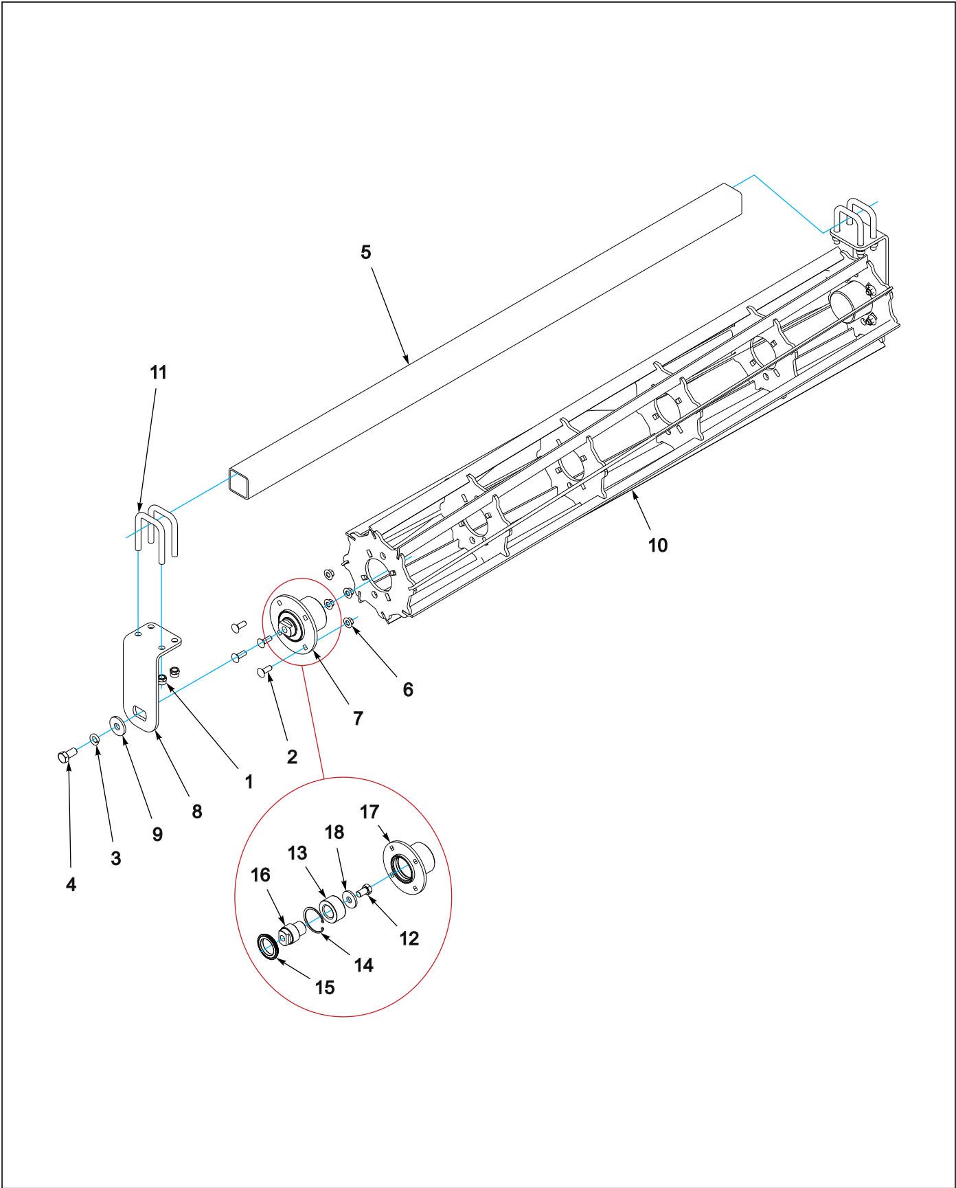
Figure 1-37: Flat Reel Assembly
