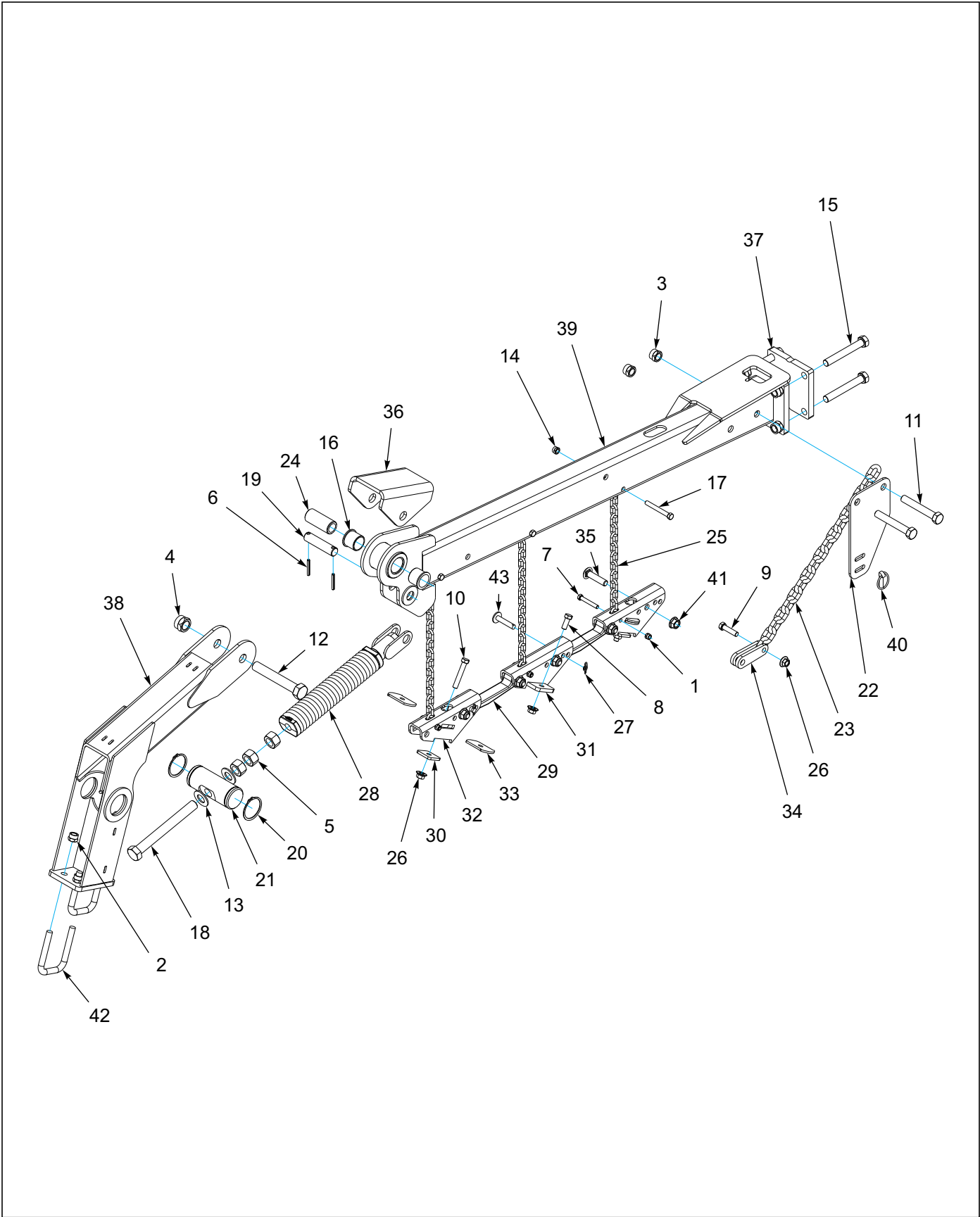
Figure 1-39: Arm Assembly - Spike & Reel
