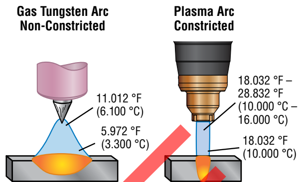
Figure 2 – TIG and Plasma Arcs
