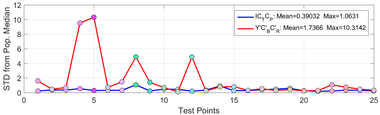
Figure 9: Objective analysis of the uniformity of MacAdam ellipses
