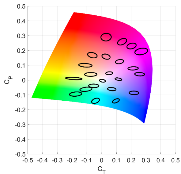
Figure 8: IC_TCP JND analysis
