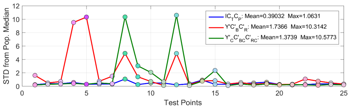
Figure 12: MacAdam JND uniformity comparison
