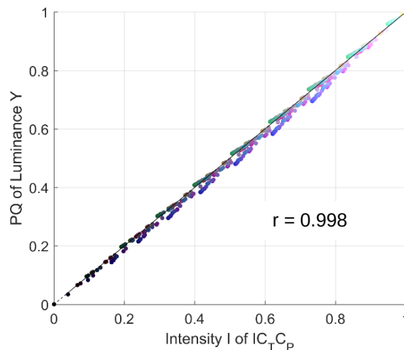
Figure 2: IC_T C_P luminance analysis
