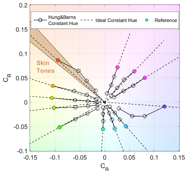
Figure 5: PQ based BT.2020 NCL Y'C'_B C'_R Hung & Berns hue linearity analysis
