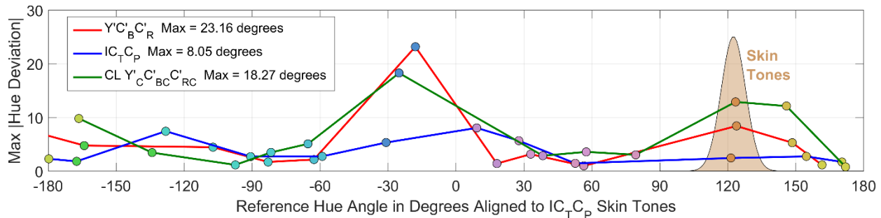
Figure 11: Hung and Berns maximum hue angle deviation comparison
