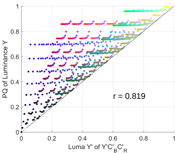
Figure 3: PQ based BT.2020 NCL Y'C'_B C'_R luminance analysis
