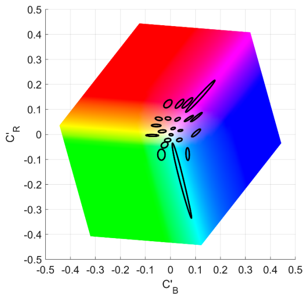
Figure 7: PQ based BT.2020 NCL Y'C'_BC'_R JND analysis
