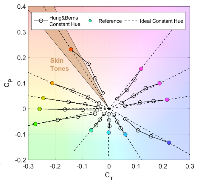
Figure 6: IC_T C_P Hung & Berns hue linearity analysis
