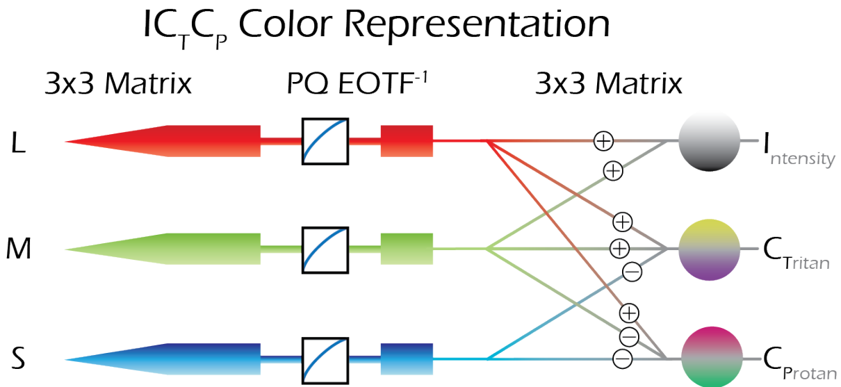
Figure 1: IC_{TC_P} and the relationship to the Human Visual System
