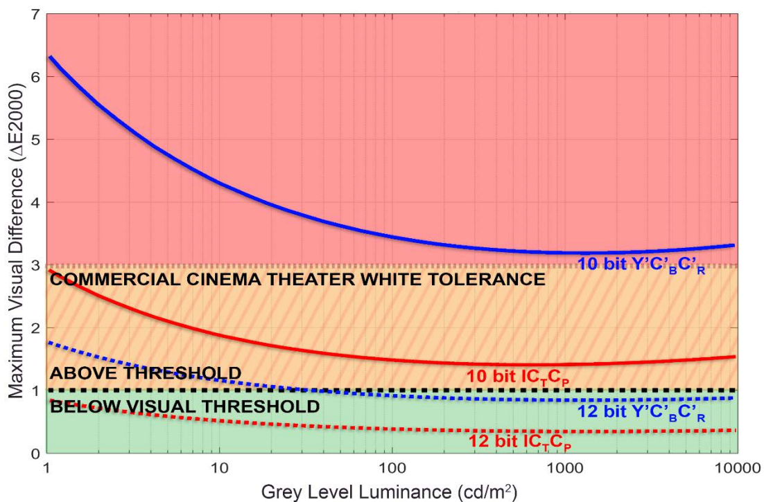
Figure 10: Baseband quantization comparison at 10 and 12 bits
