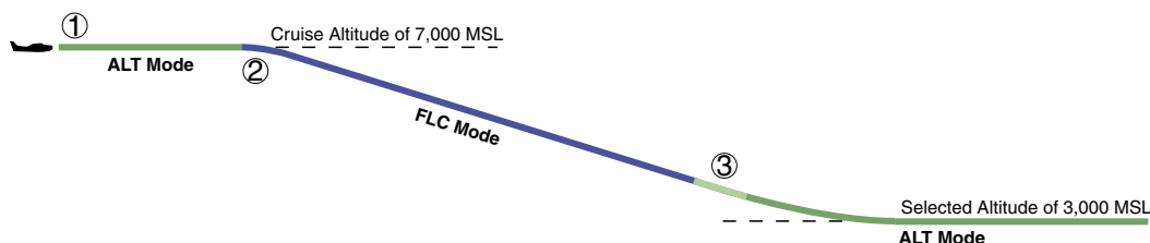
Figure 6-34 FLC Descent
