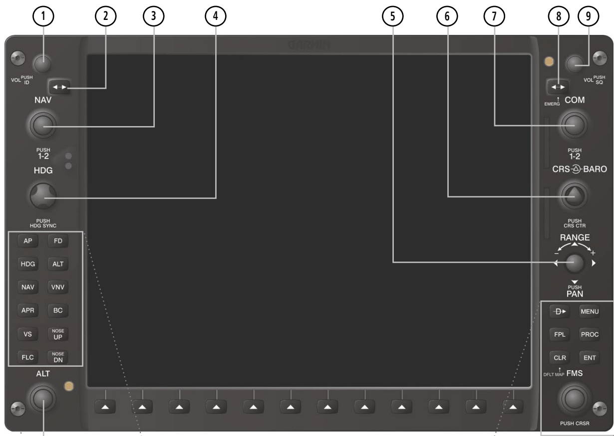
Figure 1-1 PFD/MFD Controls
