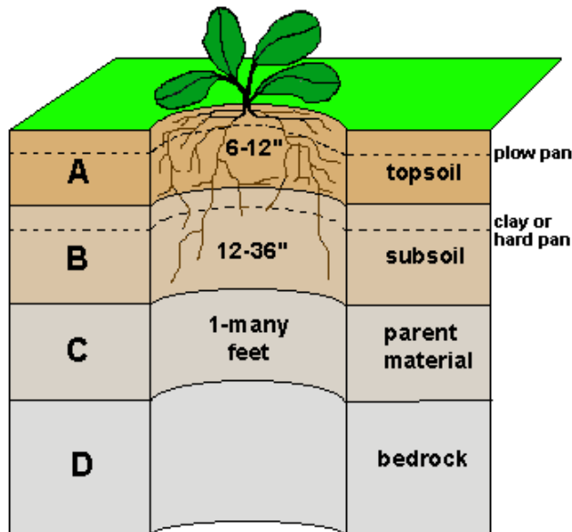
Figure 2.4 Soil Horizons.
